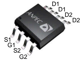
Top View of SOP – 8
