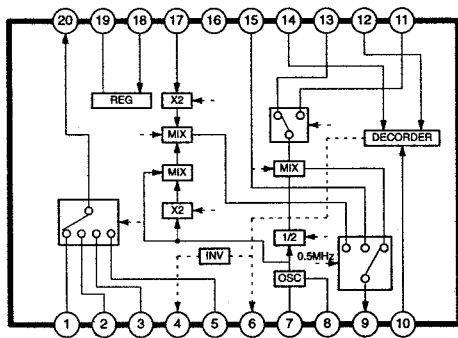
IC203 (VIDEO / AUDIO SIGNAL SELECT SWITCH : M52317SP)
