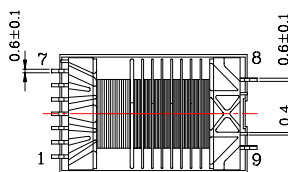
<< EEL-19 BOTTOM VIEW >>
