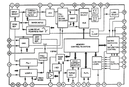
A BOARD IC301 MC4402P/MC4407P
