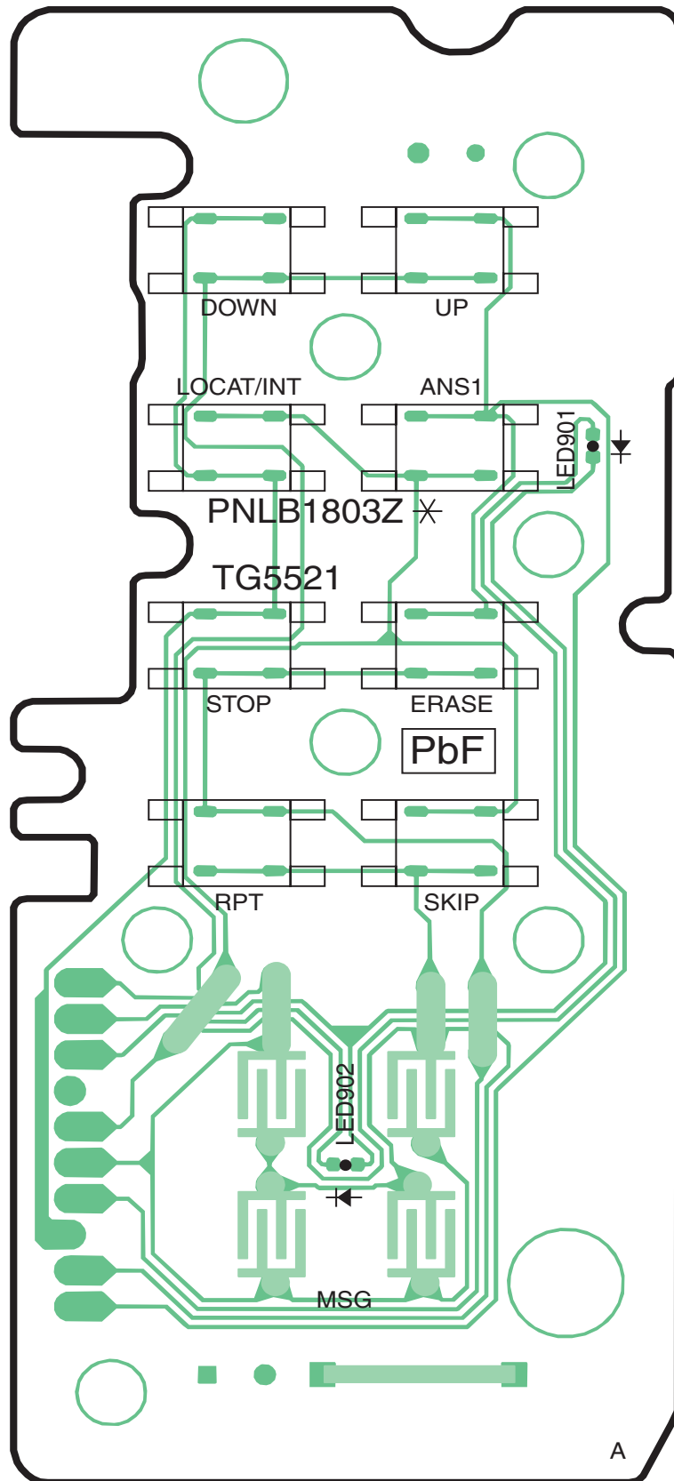
KX-TG5521 CIRCUIT BOARD (Base Unit_Operation (Component View))
