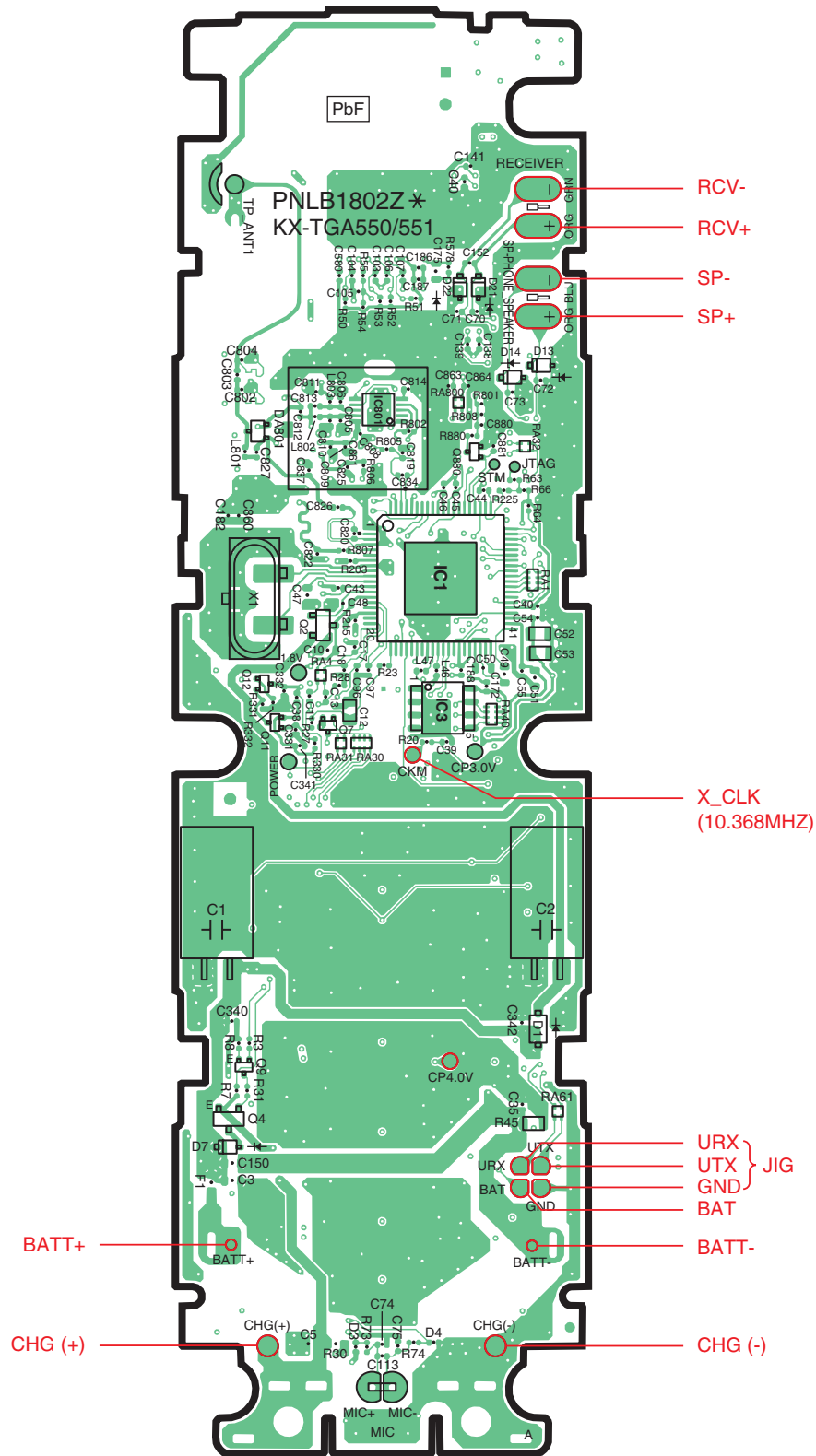
KX-TGA551 CIRCUIT BOARD (Handset_Main (Component View))
