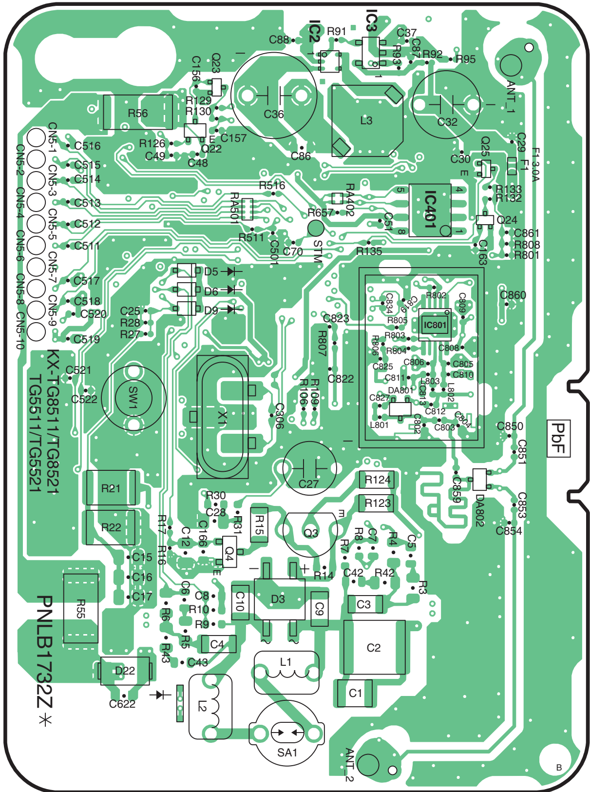
KX-TG5521 CIRCUIT BOARD (Base Unit_Main (Component View))
