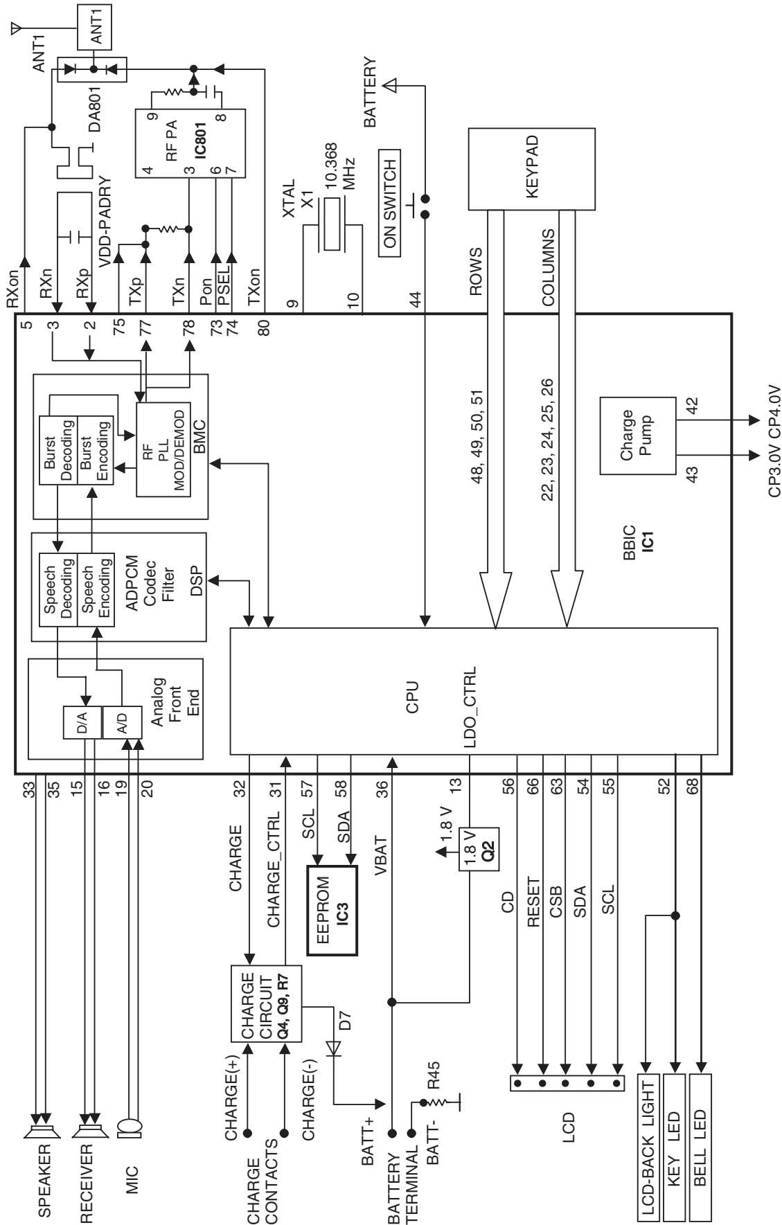
KX-TGA551 BLOCK DIAGRAM (HANDSET)
