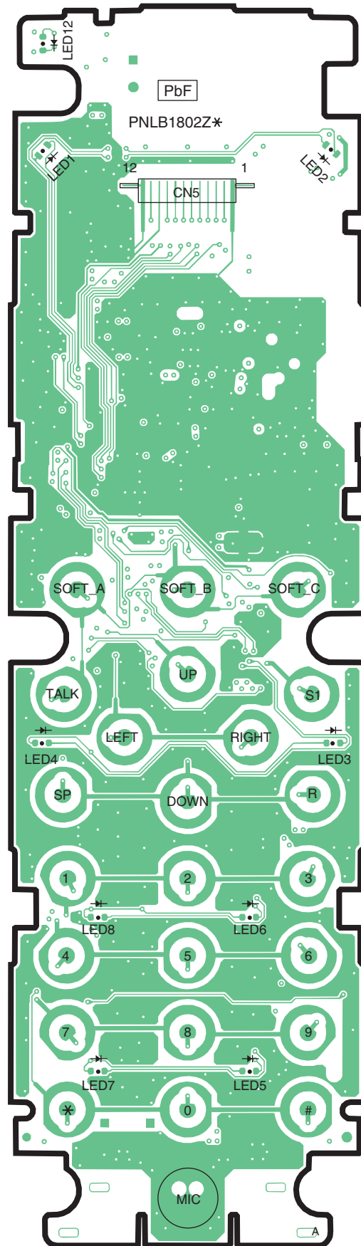
KX-TGA551 CIRCUIT BOARD (Handset_Main (Bottom View))
