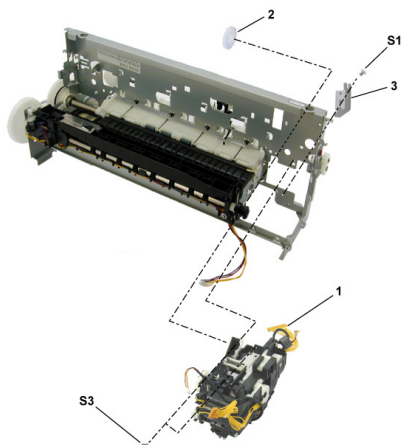
FIGURE 11 PAPER FEED & CARRIAGE LIFT PART
