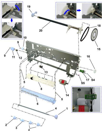
FIGURE 11 PAPER FEED & CARRIAGE LIFT PART
