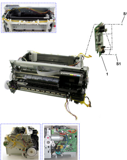
FIGURE 5 LOGIC BOARD ASS'Y
