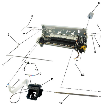
FIGURE 8 CARRIAGE UNIT
