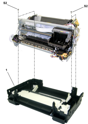
FIGURE 6 SHEET FEED UNIT
