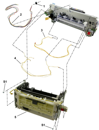
FIGURE 6 SHEET FEED UNIT
