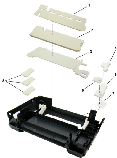
FIGURE 9 PURGE UNIT
