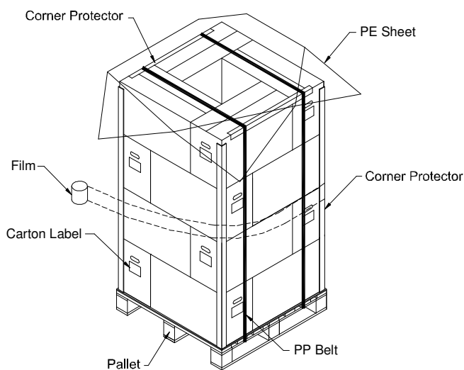
Figure. 8-2 packing method
