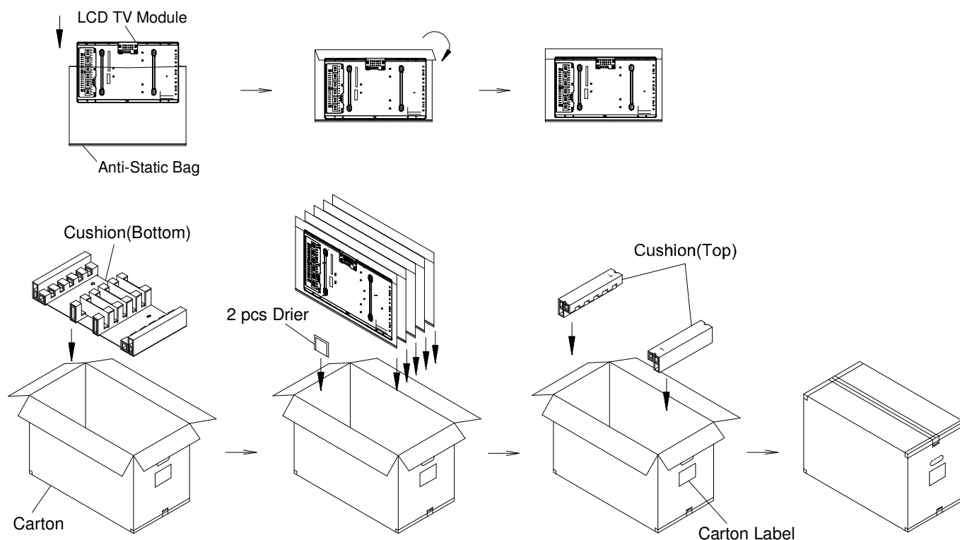
Figure.8-1 packing method
