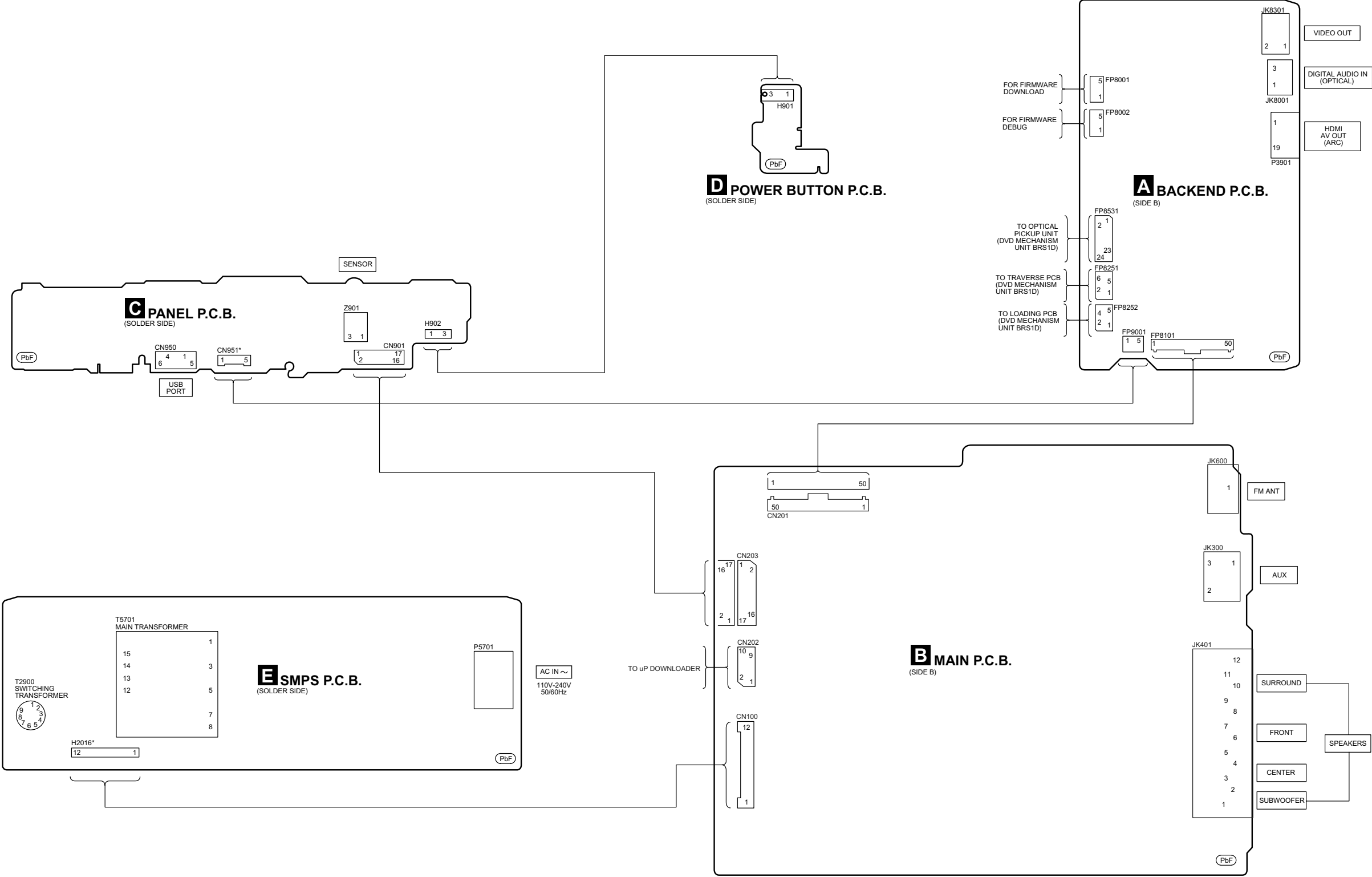
SA-XH70PH WIRING CONNECTION DIAGRAM
