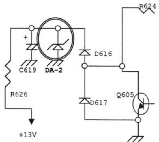
A2-SCHEMATIC DIAGRAM AFTER MODIF.
