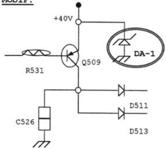
A1-SCHEMATIC DIAGRAM AFTER MODIF.
