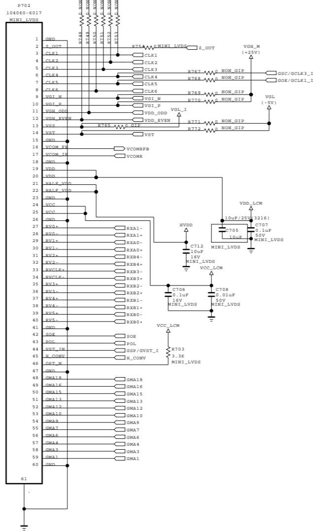
[Right FFC Connector] (60Pin Mini-LVDS)
