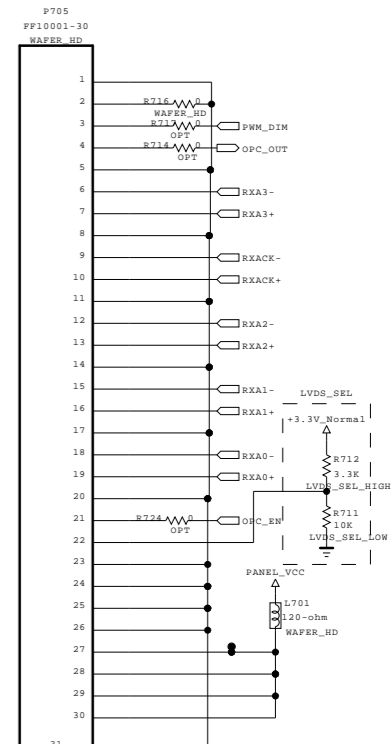
[30Pin LVDS Connector] (For HD 60Hz_Normal)
