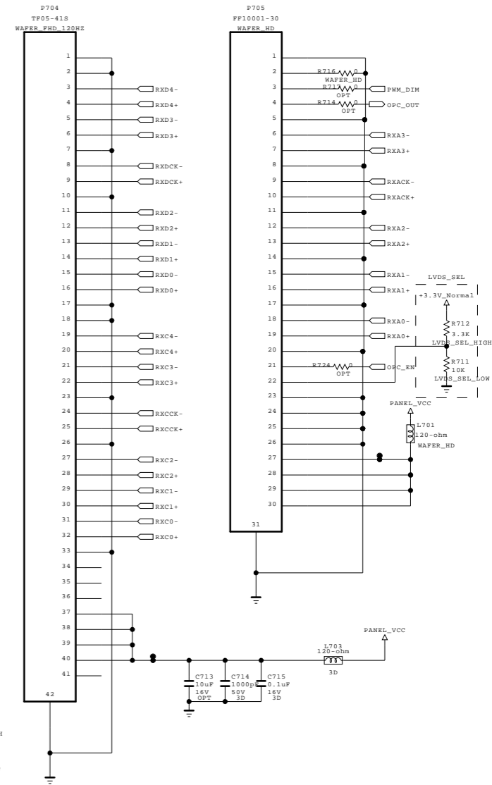
[41Pin LVDS Connector] (For FHD 120Hz)
