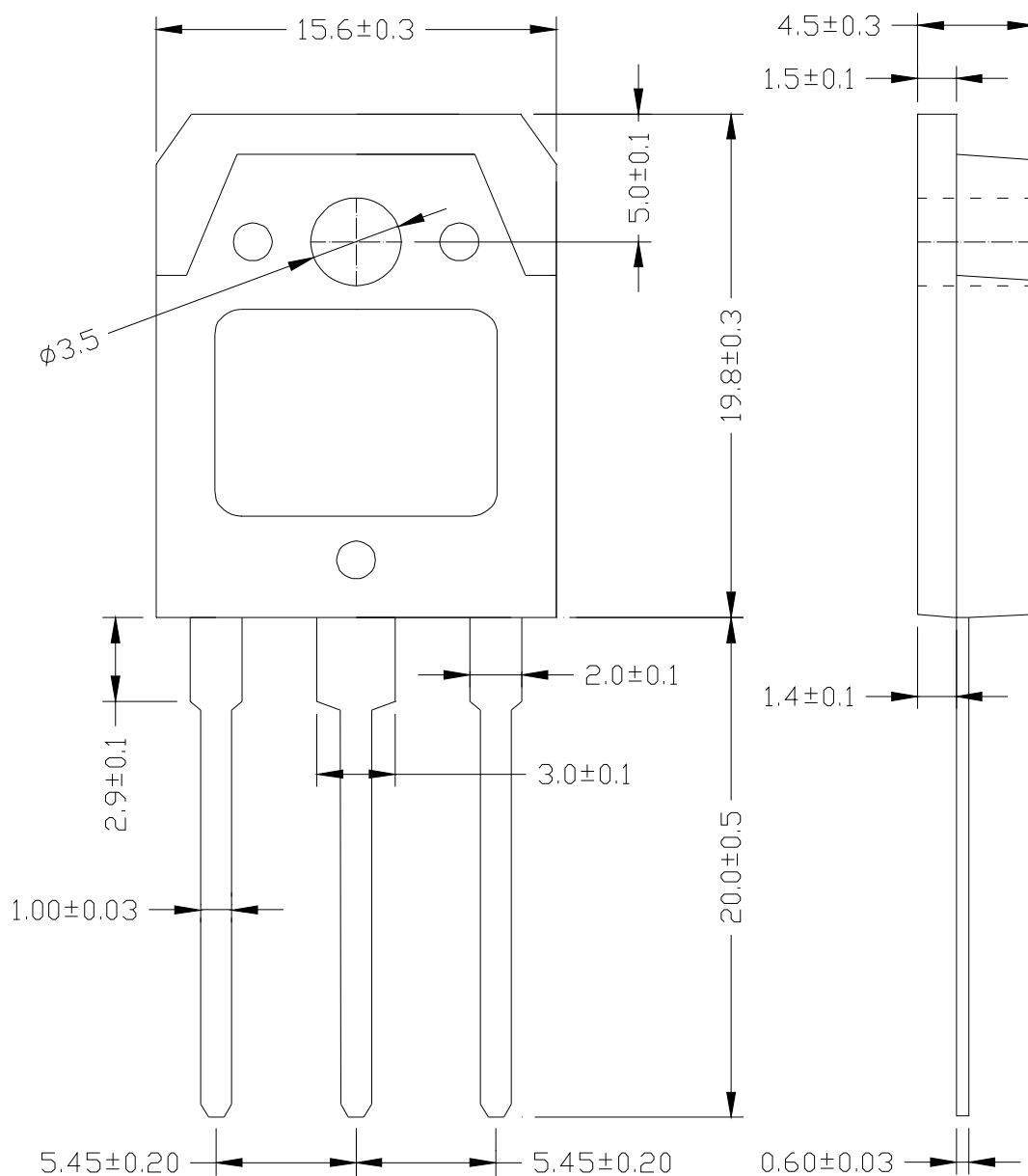
TO-3PB
