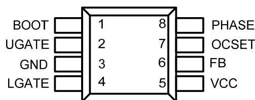
Figure 1. Pin Assignment of FP6321
