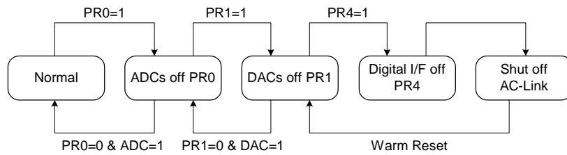
Figure 20. STAC9750/51 Powerdown/Powerup flow with analog still alive
