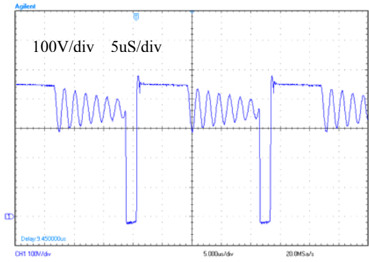
Vin=265V, Io=0.5A
