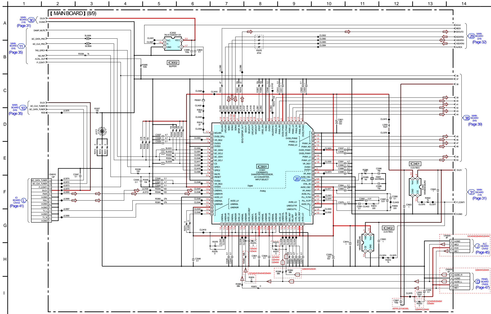
5-15. SCHEMATIC DIAGRAM – MAIN Section (8/9) – • See page 28 for waveform. • See page 61 for IC Pin Function Description of IC3001.
