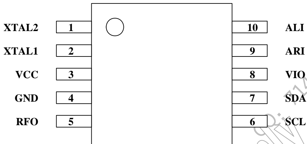
Figure 2: QN8027 Device Pin Out
