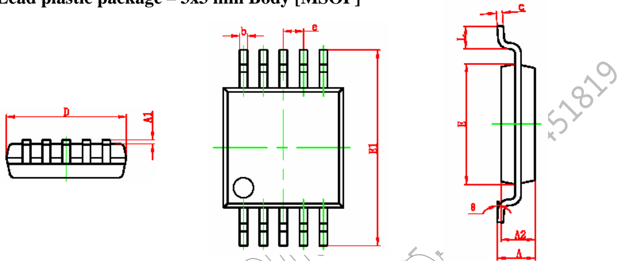
Figure 5: MSOP10 Package Outline Dimensions
