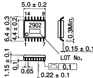
BA2902FV(SSOP-B14) (Unit:[mm])
