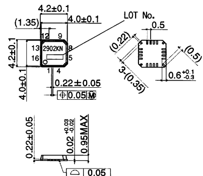
BA2902KN(VQFN16) (Unit:[mm])
