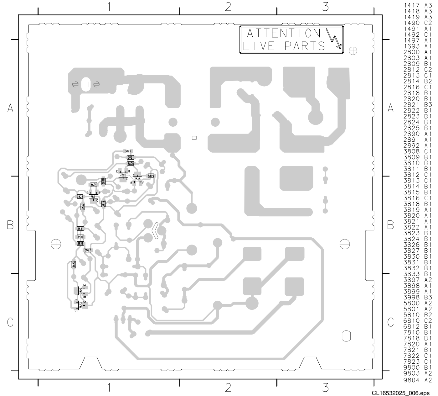
Layout DAF Panel (Bottom View)
