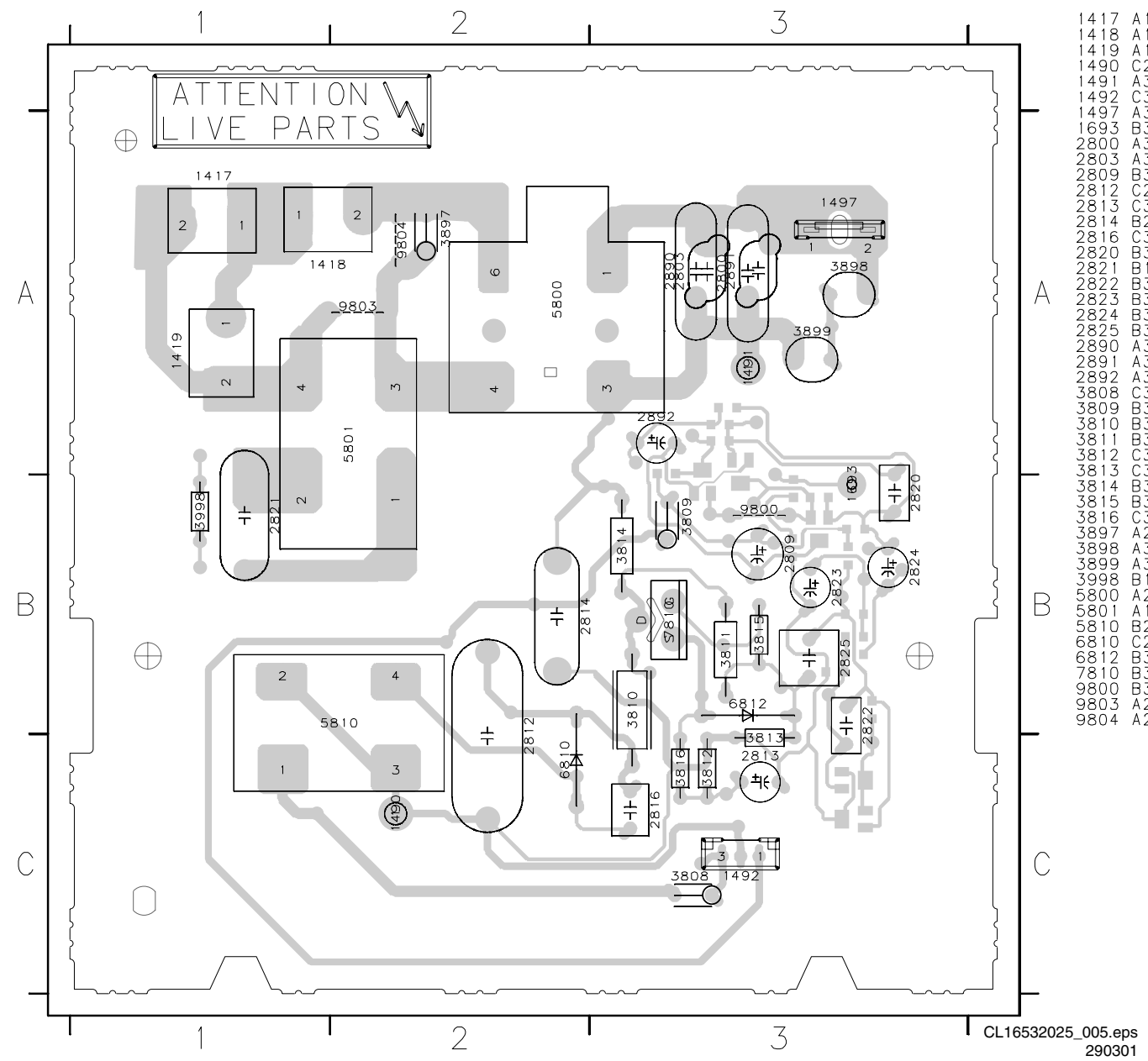
Layout DAF Panel (Top View)
