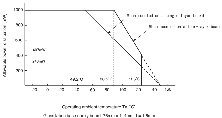
Glass fabric base epoxy board 76mm × 114mm t = 1.6mm
