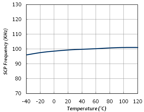
SCP Frequency vs. Temperature
