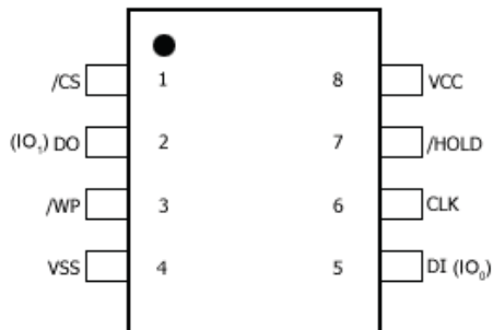
PIN CONFIGURATION PDIP 300-MIL
