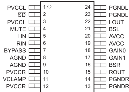
PWP (TSSOP) PACKAGE (TOP VIEW)
