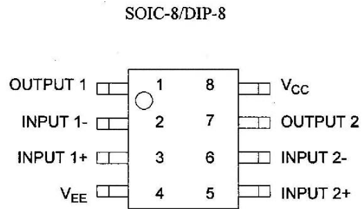
Figure 2. Pin Configuration of LM4558 (Top View)
