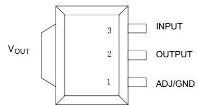
U Package (SOT-89)
