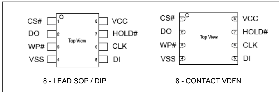
Figure.1 CONNECTION DIAGRAMS
