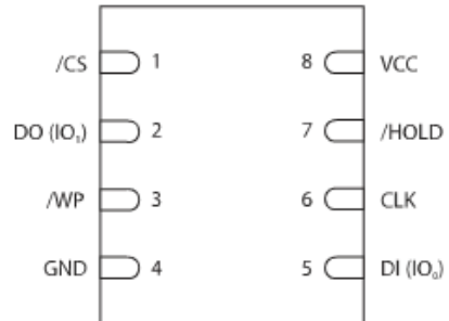
PAD CONFIGURATION WSON 6X5-MM
