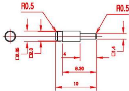
SOLDER PIN S:2/1
