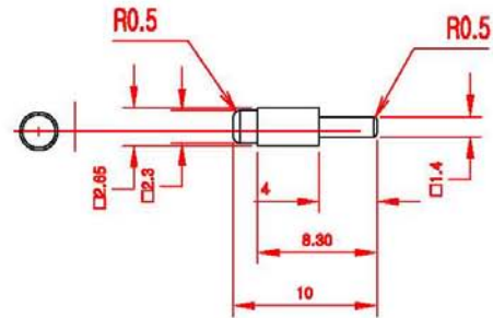
SOLDER PIN
