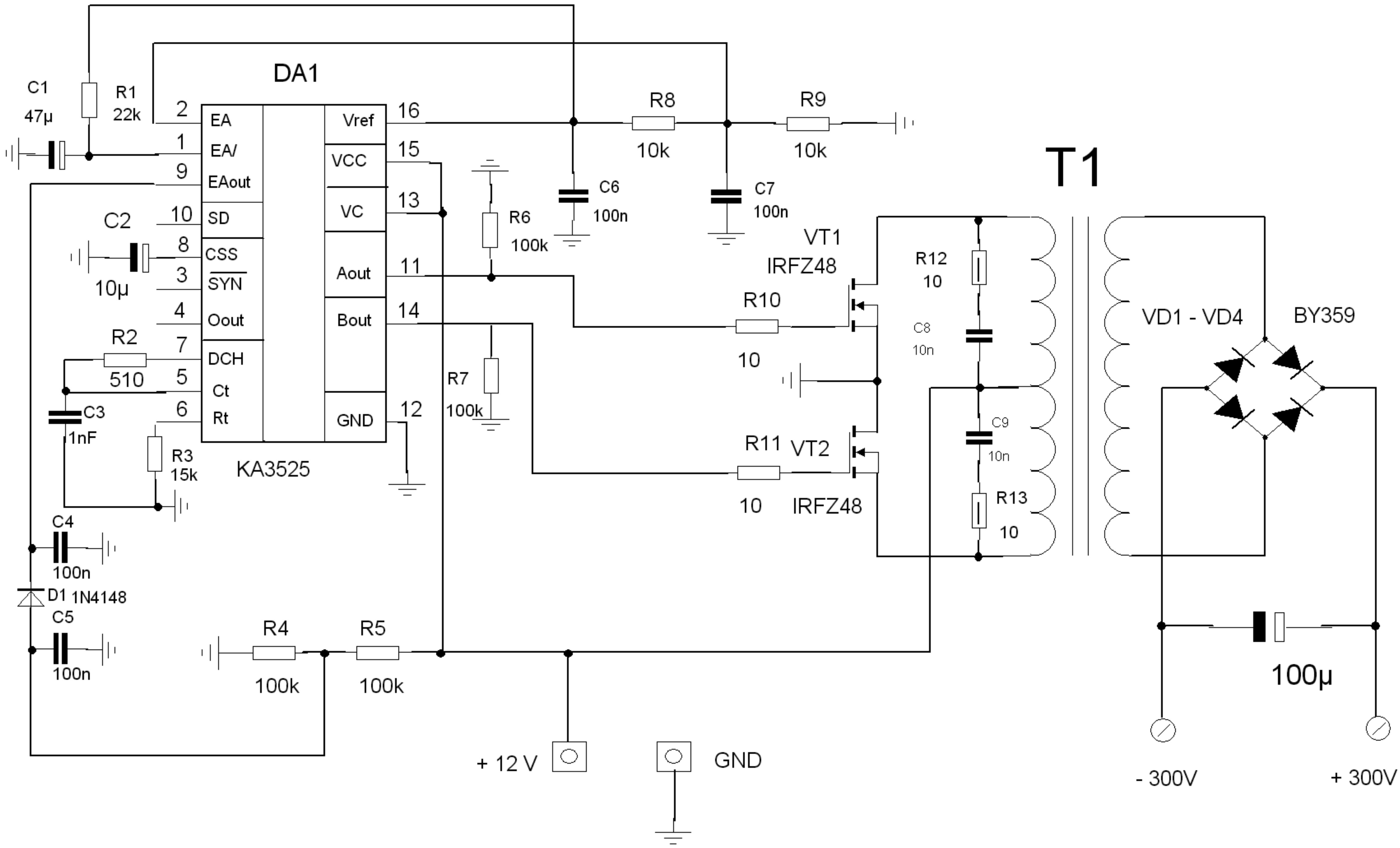
DC / AC CONVERTER VOLTAGE + 12V / ~300V
