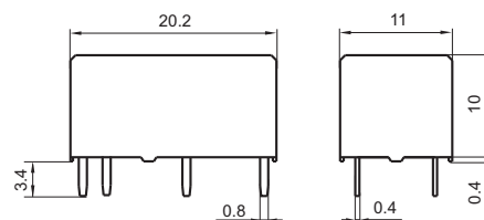
2 coils latching
