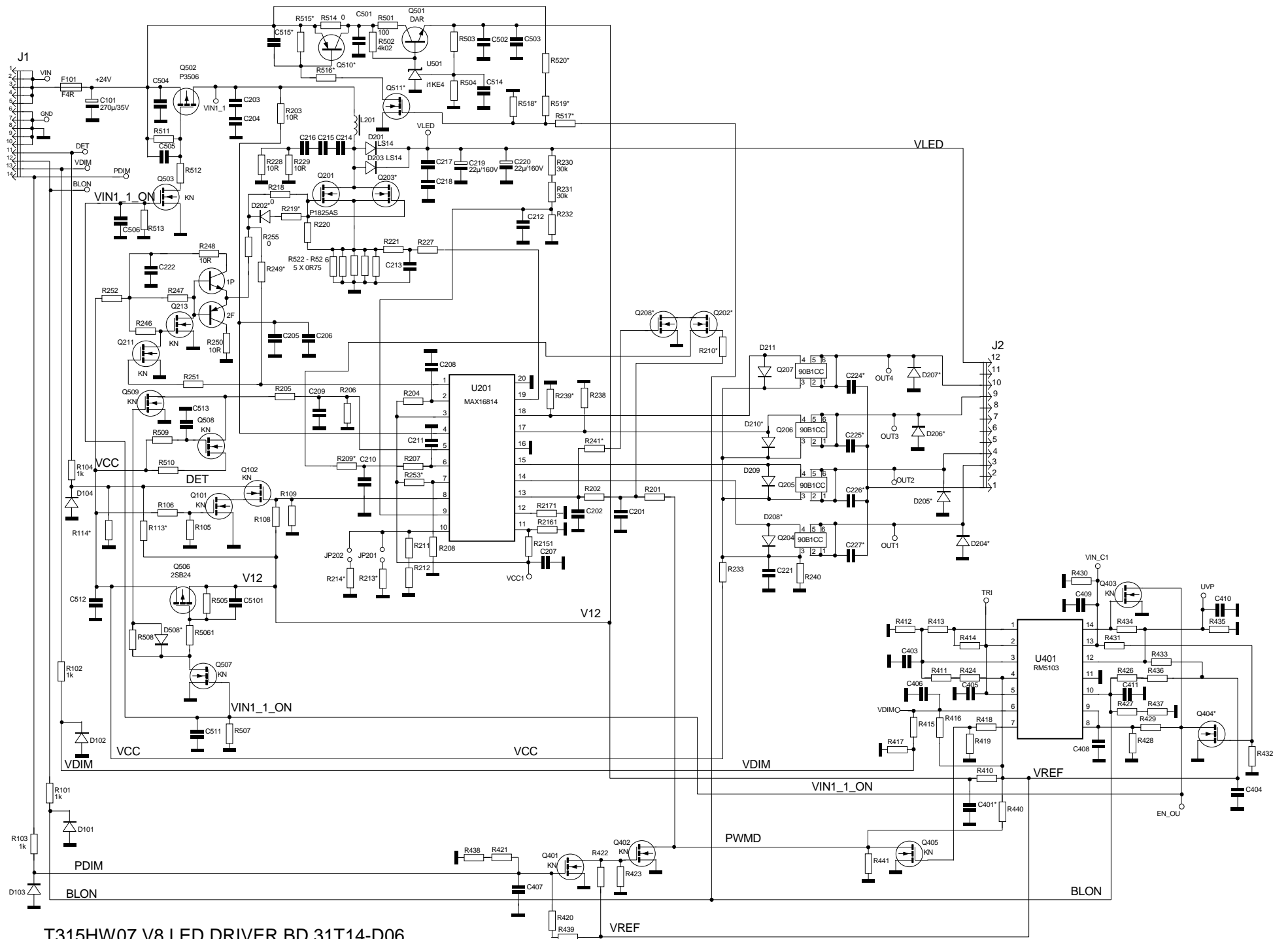
T315HW07 V8 LED DRIVER BD 31T14-D06
