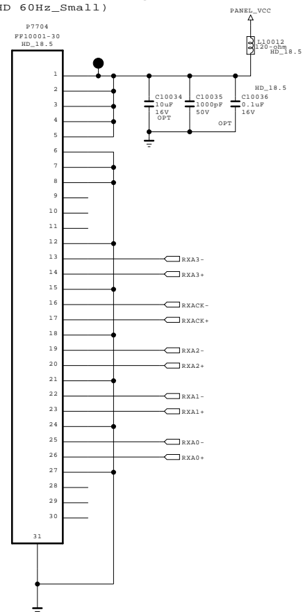
[30Pin HD LVDS Connector] (For HD 60Hz_Small)
