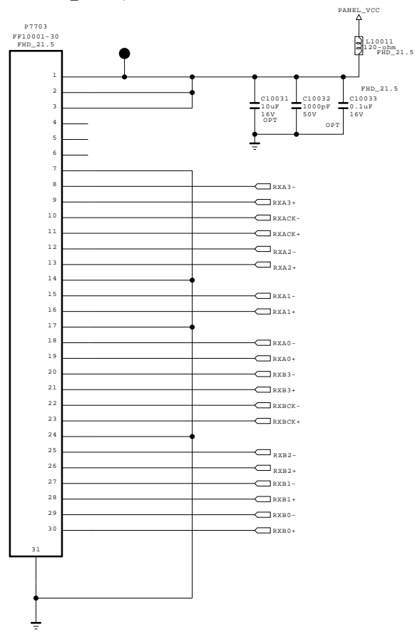
[30Pin FHD LVDS Connector] (For FHD 60Hz_Small)
