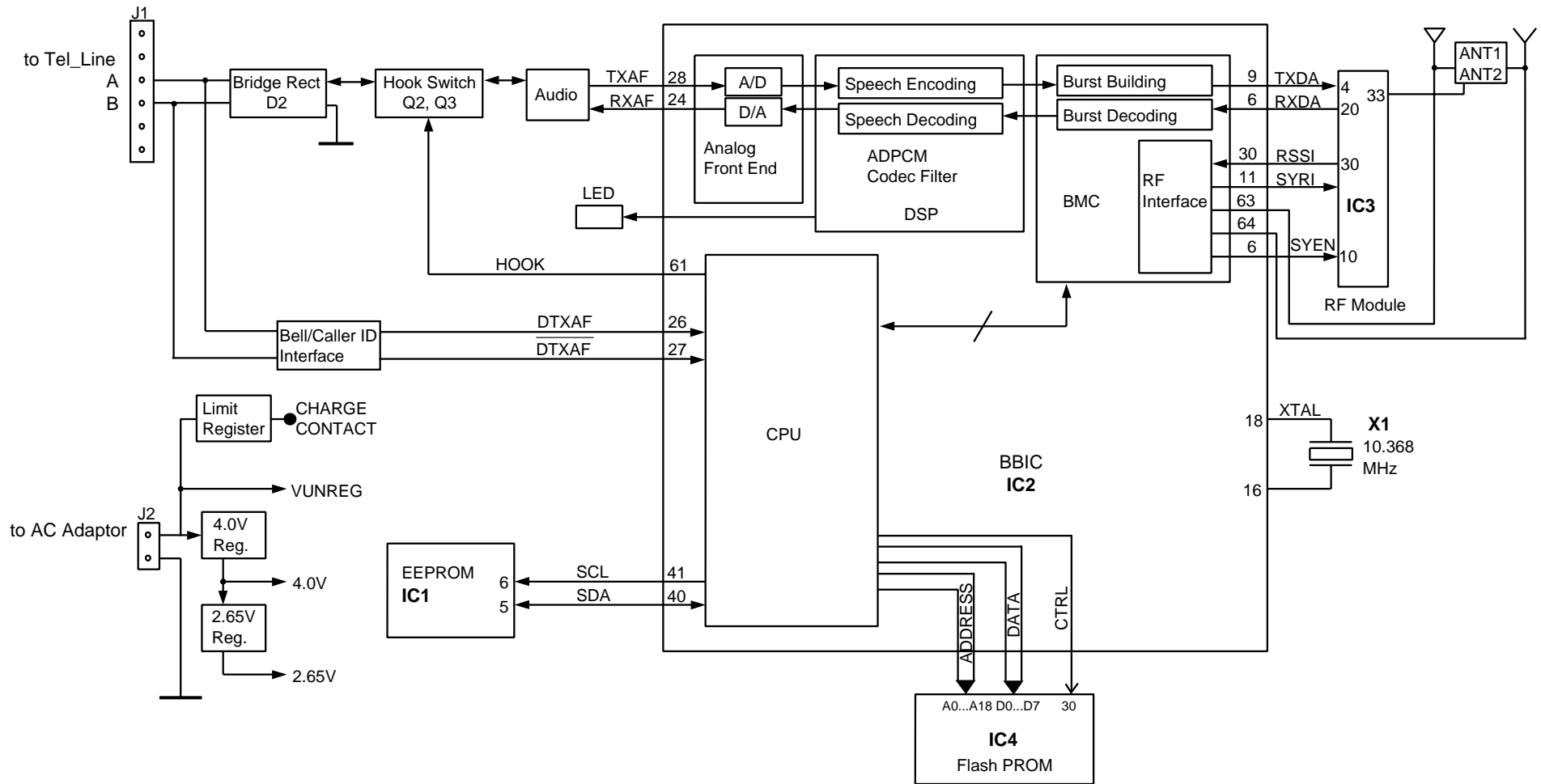
KX-TCD410RUM/RUS&412RUM/RUS BLOCK DIAGRAM (BASE UNIT)
