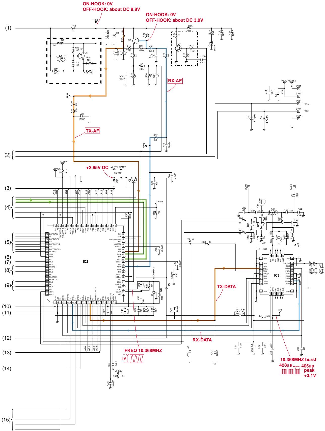
KX-TCD410RUM/RUS&412RUM/RUS SCHEMATIC DIAGRAM (BASE UNIT)
