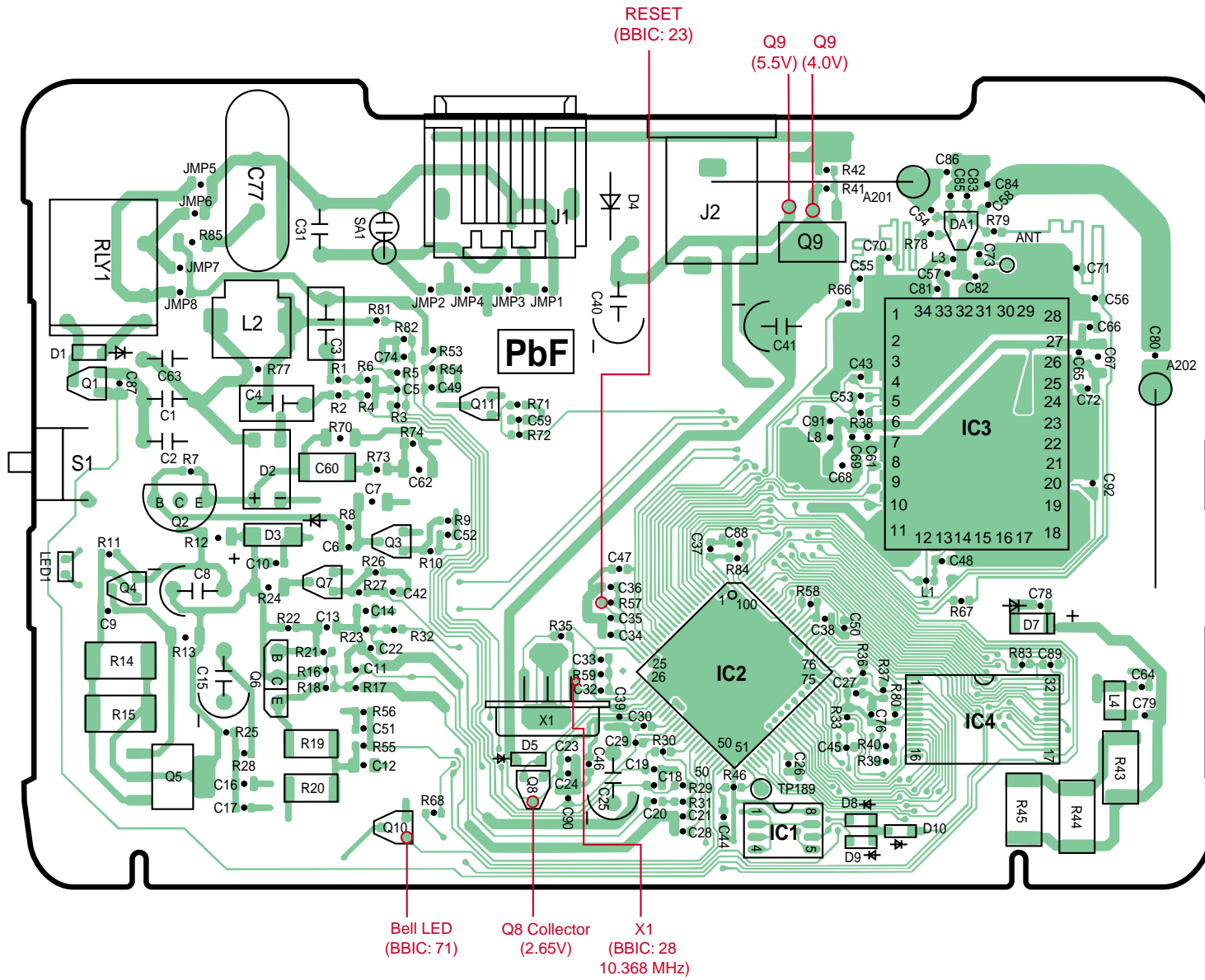
KX-TCD410RUM/RUS&412RUM/RUS CIRCUIT BOARD (BASE UNIT) Component View
