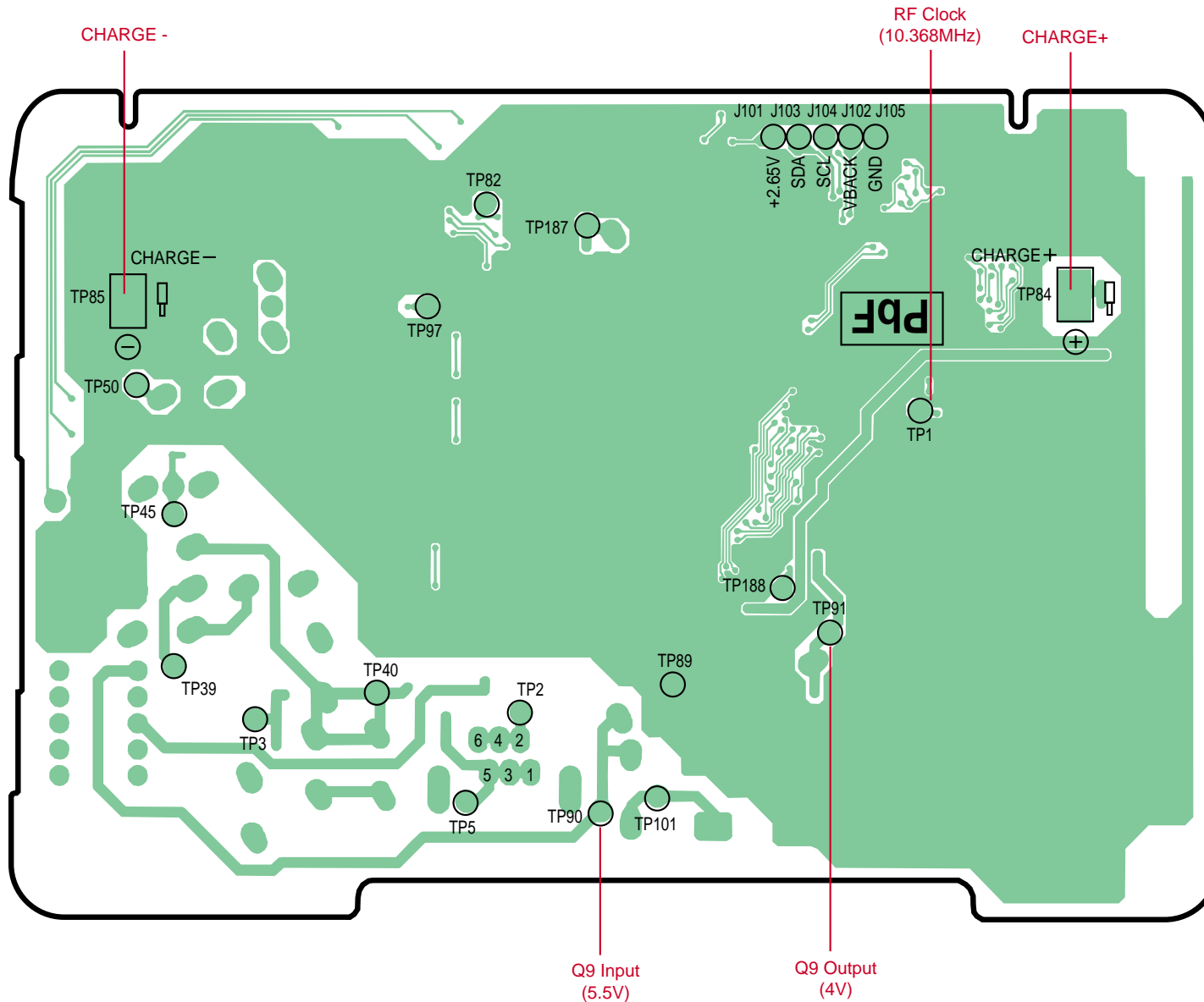
KX-TCD410RUM/RUS&412RUM/RUS CIRCUIT BOARD (BASE UNIT) Flow Solder Side View
