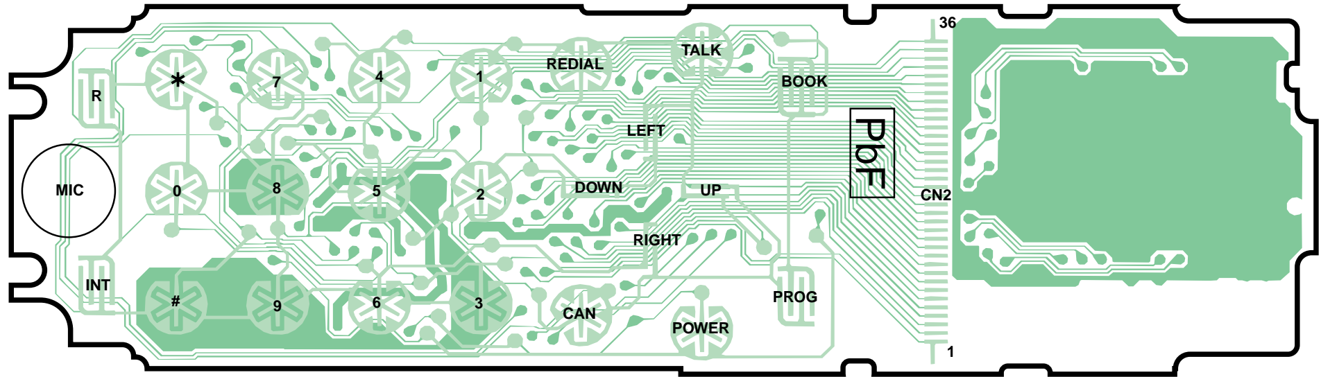
KX-A141RUM/RUS&142RUM/RUS CIRCUIT BOARD (HANDSET) Flow Solder Side View
