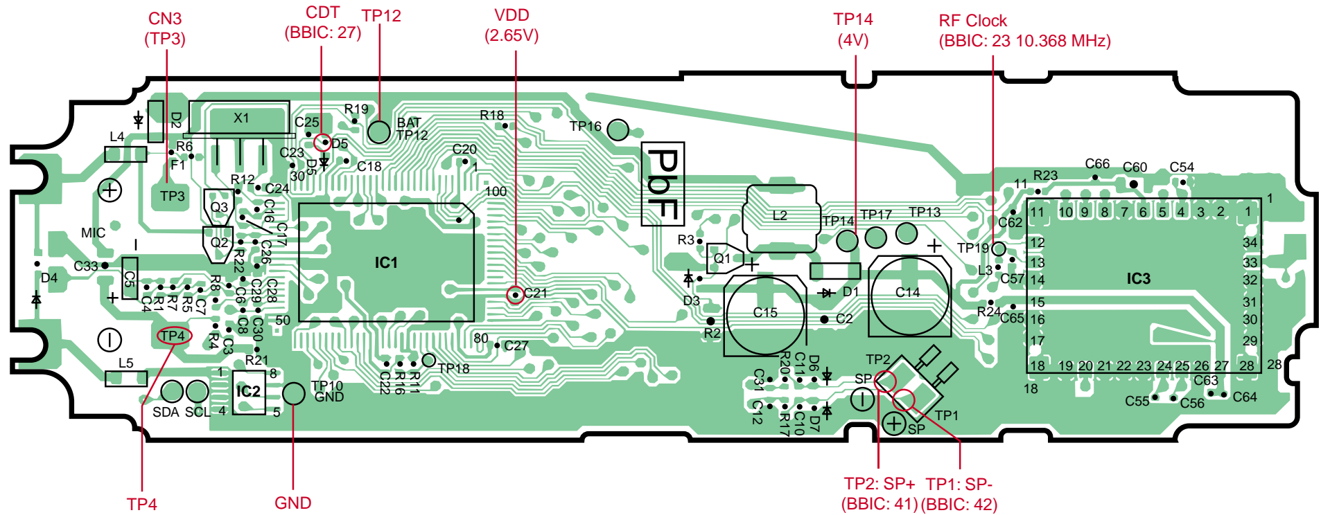
KX-A141RUM/RUS&142RUM/RUS CIRCUIT BOARD (HANDSET) Component View
