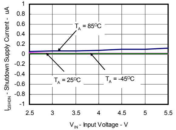
Shutdown Supply Current vs. Input Voltage
