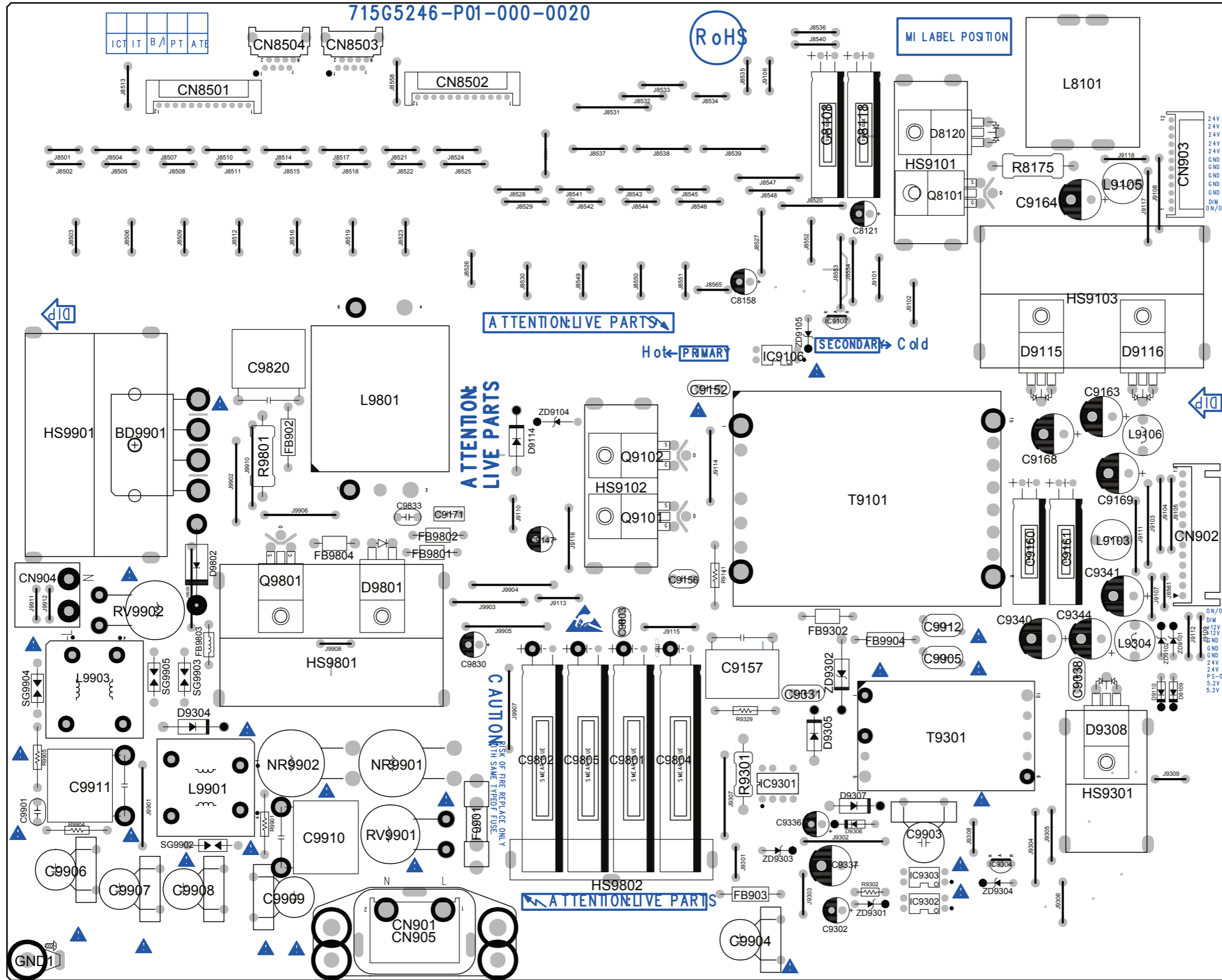
10-2-4 Power layout top
