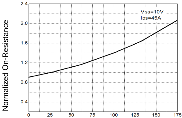
Figure 7: On-Resistance vs. Temperature
