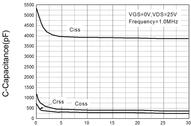
Figure 9: Capacitance Characteristics
