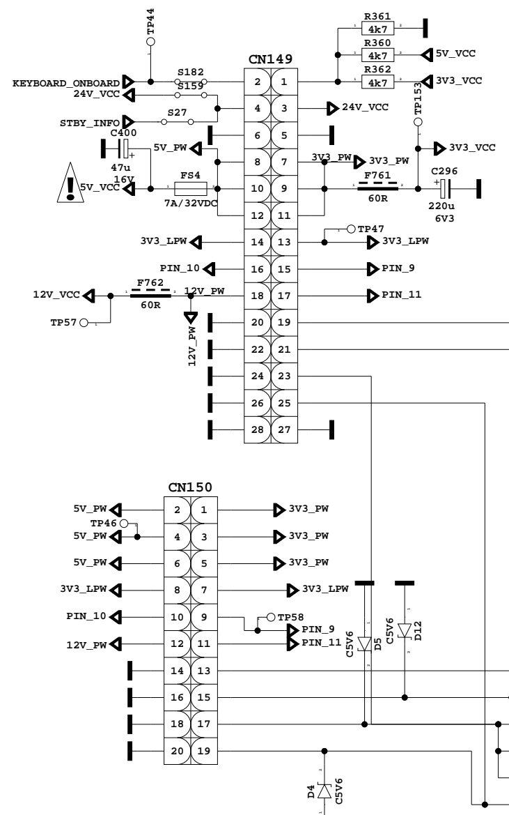
17IPS15 CONNECTOR
