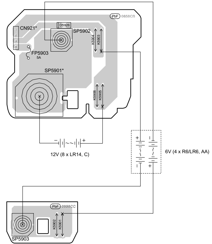
I BATTERY (2) P.C.B. (REPNT0063H)
