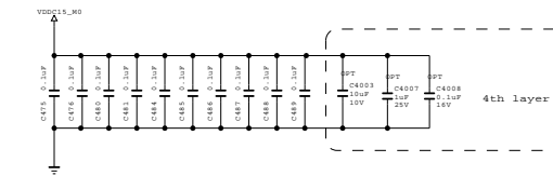
+1.5V_Bypass Cap Close to DDR Power Pin
