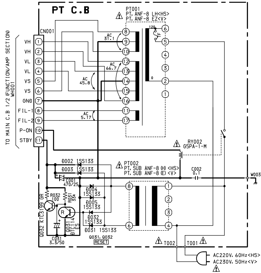
SCHEMATIC DIAGRAM-5 [PT]
