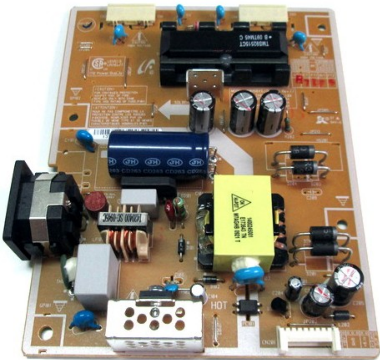
SAMSUNG BN44-00121J
