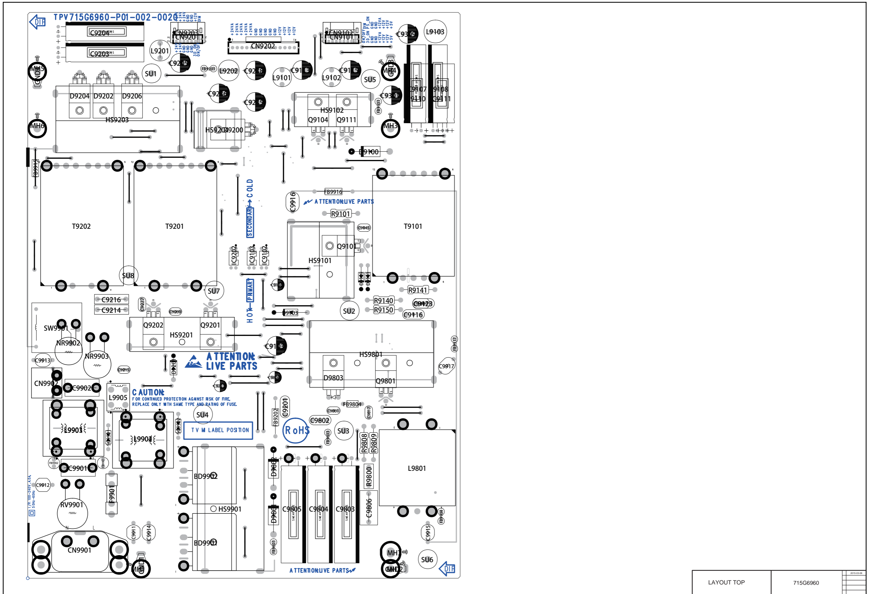
10-5-5 Power layout top
