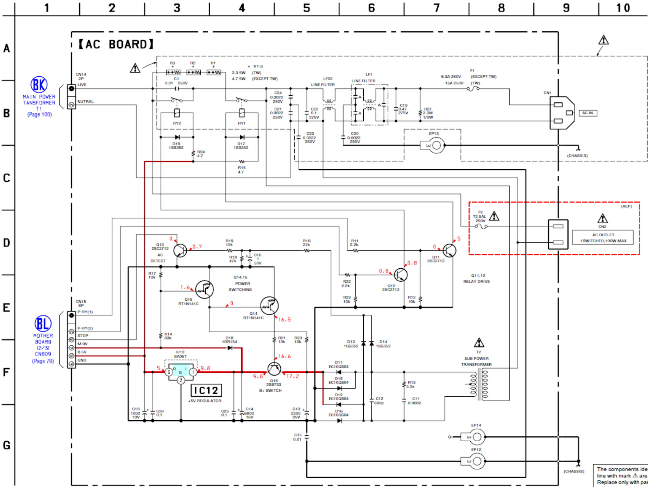
6-80. SCHEMATIC DIAGRAM – AC Board –
