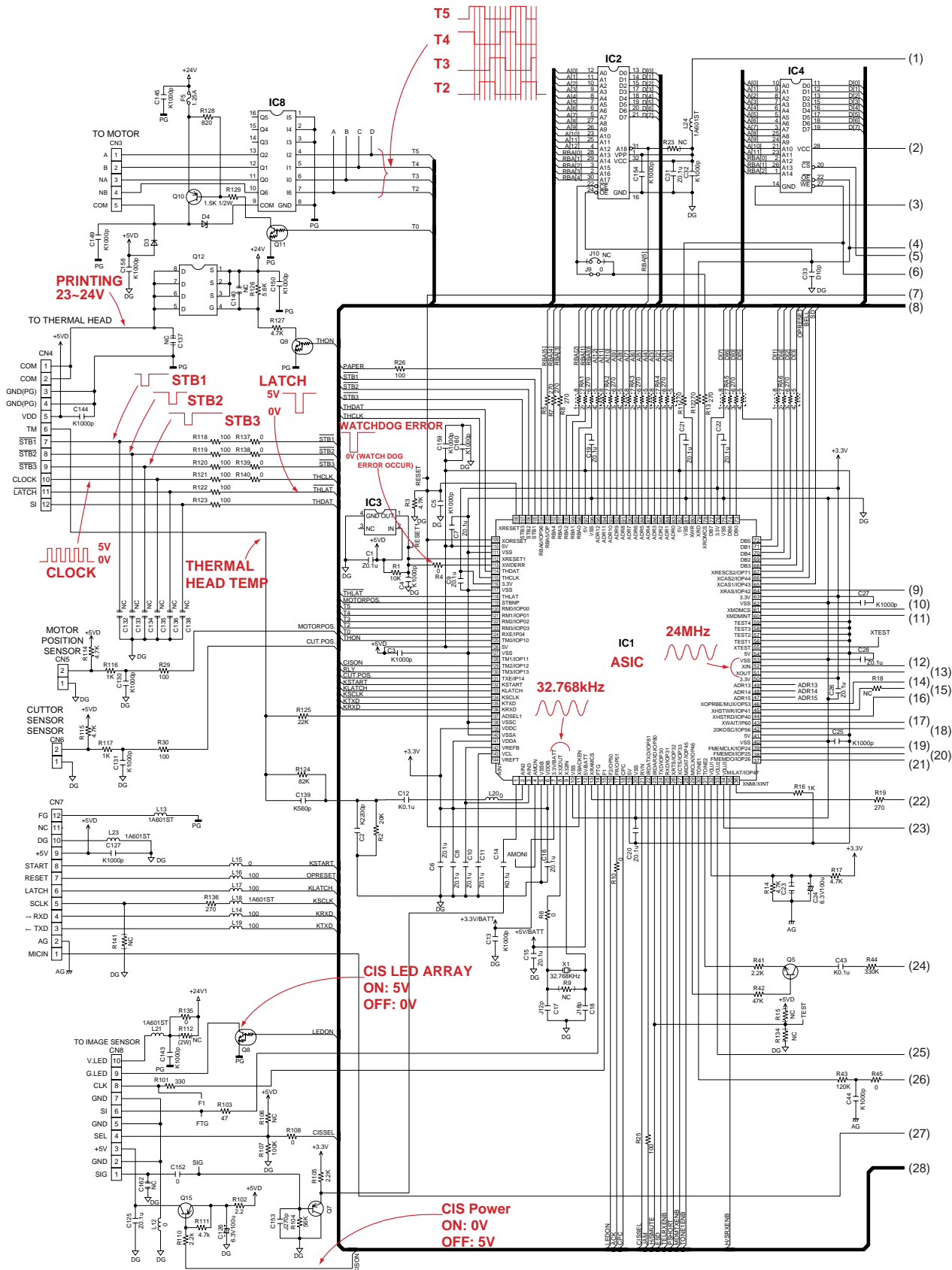
DIGITAL BOARD SCHEMATIC DIAGRAM KX-FT74RU
