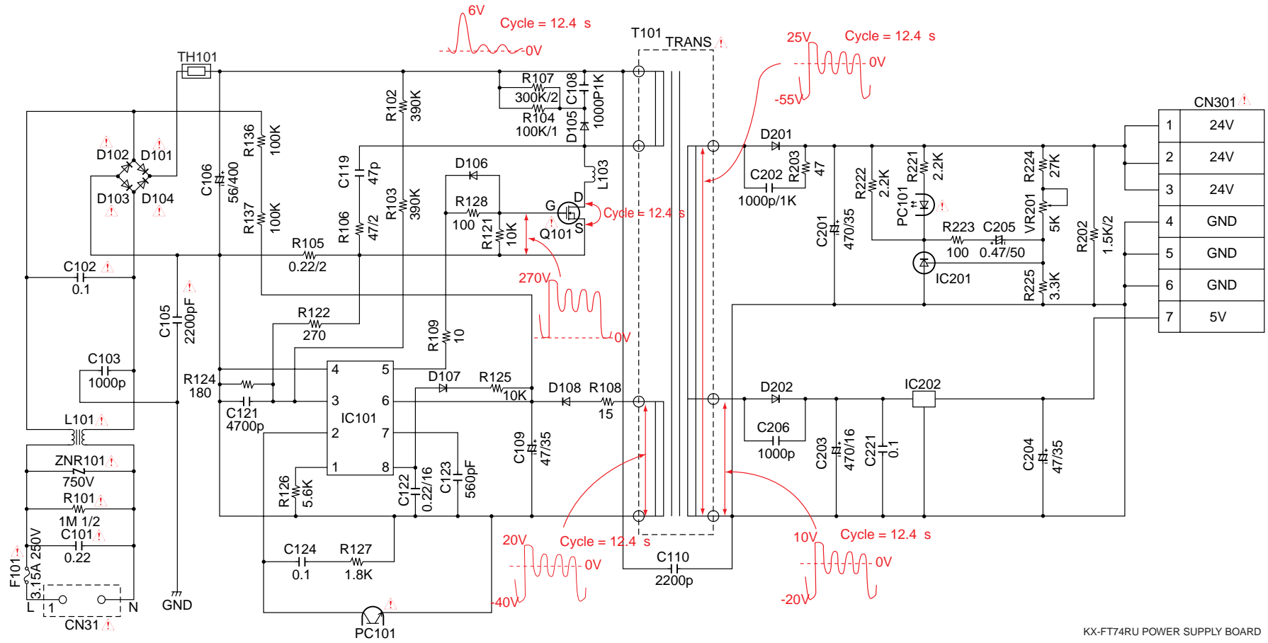
KX-FT4RU POWER SUPPLY BOARD
