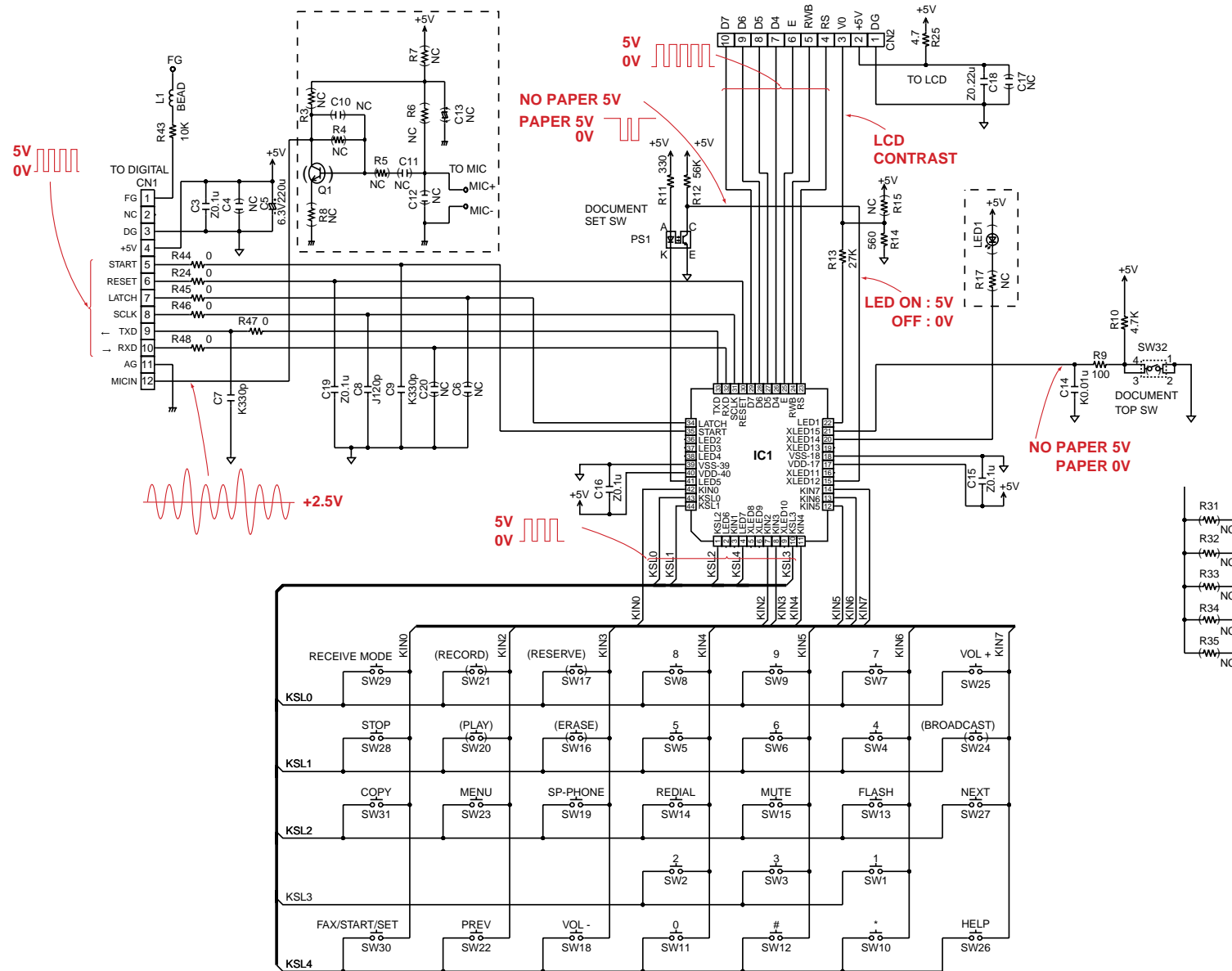
OPERATION BOARD SCHEMATIC DIAGRAM KX-FT74RU
