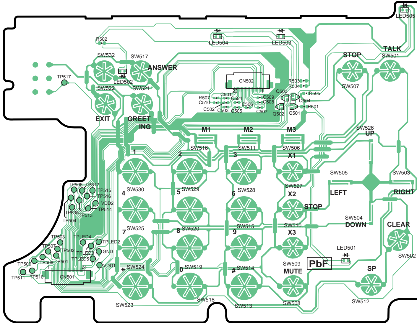
KX-TCDS30RUM/RUT CIRCUIT BOARD (BASE UNIT) Operation (Flow Solder Side View)
