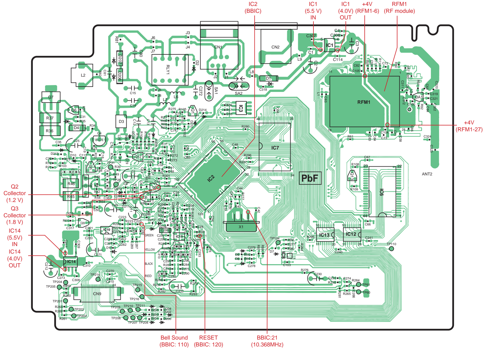
KX-TCDS30RUM/RUT CIRCUIT BOARD (BASE UNIT) Main (Component View)
