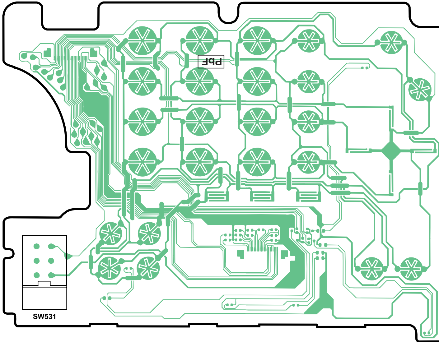
KX-TCD530RUM/RUT CIRCUIT BOARD (BASE UNIT) Operation (Component View)
