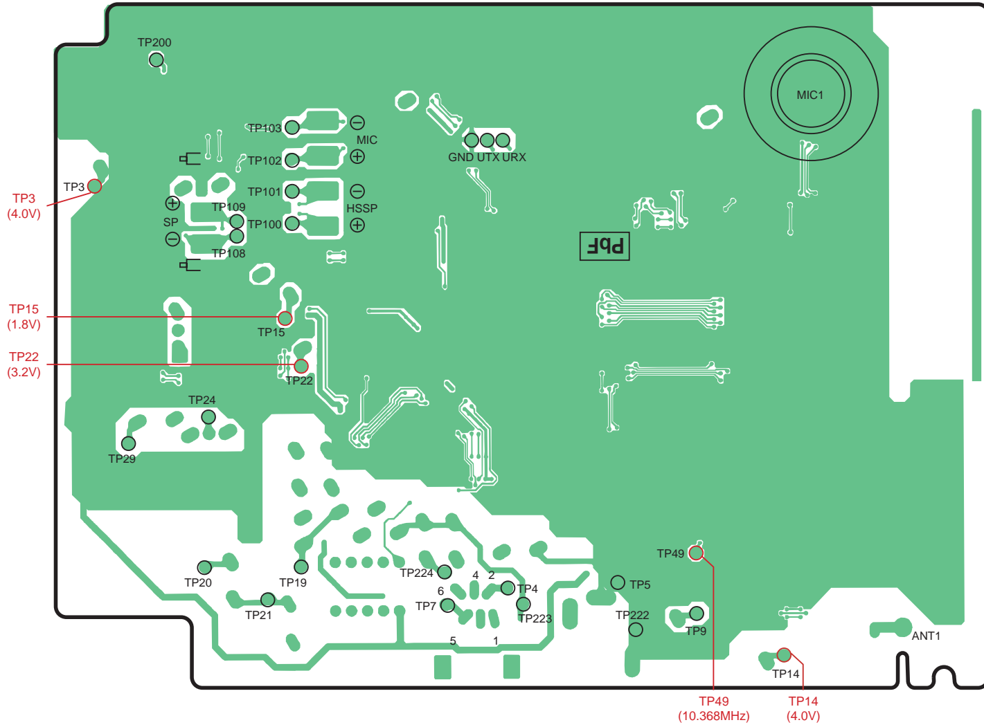
KX-TCDS30RUM/RUT CIRCUIT BOARD (BASE UNIT) Main (Flow Solder Side View)
