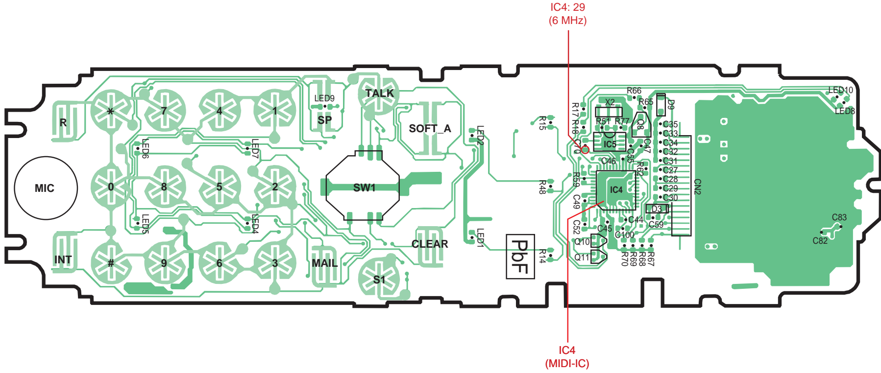
KX-TCA151RUM/RUT CIRCUIT BOARD (CORDLESS HANDSET) Flow Solder Side View
