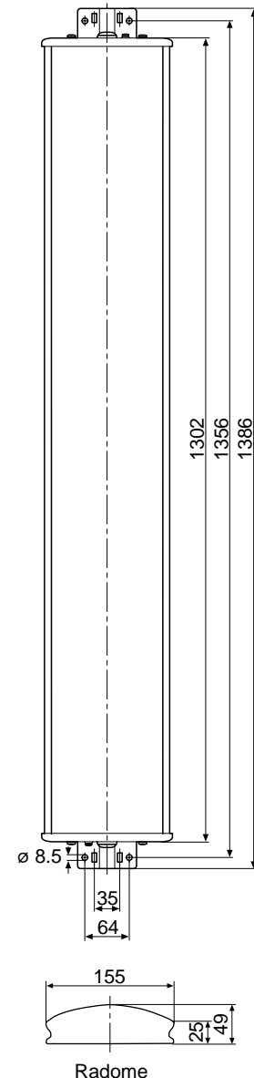
Radome
