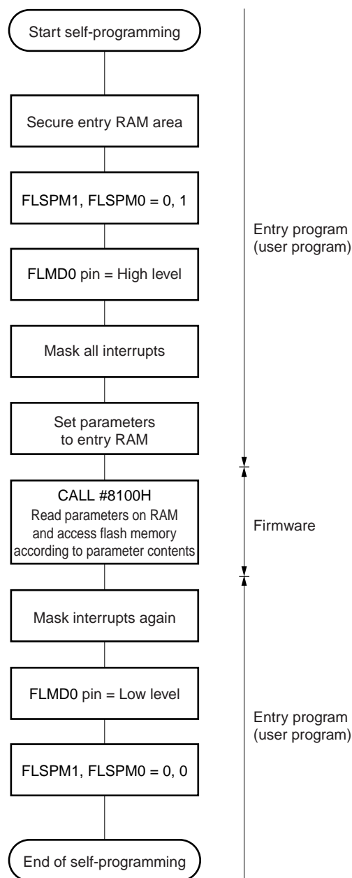
Figure 23-17. Self-Programming Procedure
