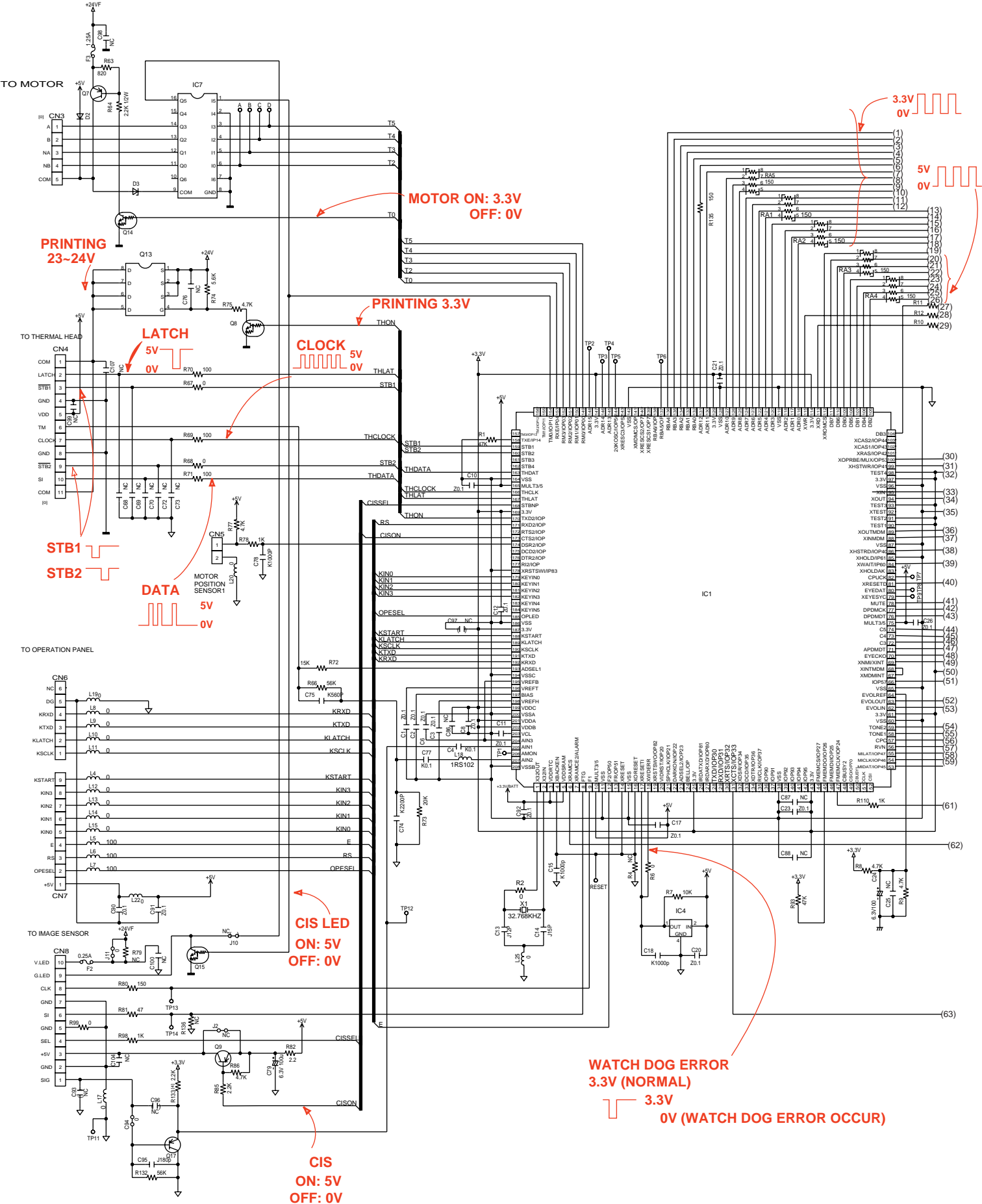
DIGITAL BOARD SCHEMATIC DIAGRAM KX-F72RU-B/W
