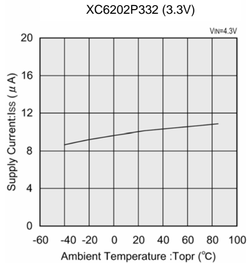
(6) Supply Current vs. Ambient Temperature
