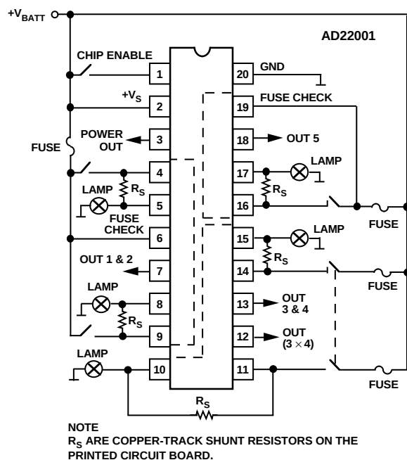
Figure 4. Application Suggestion
