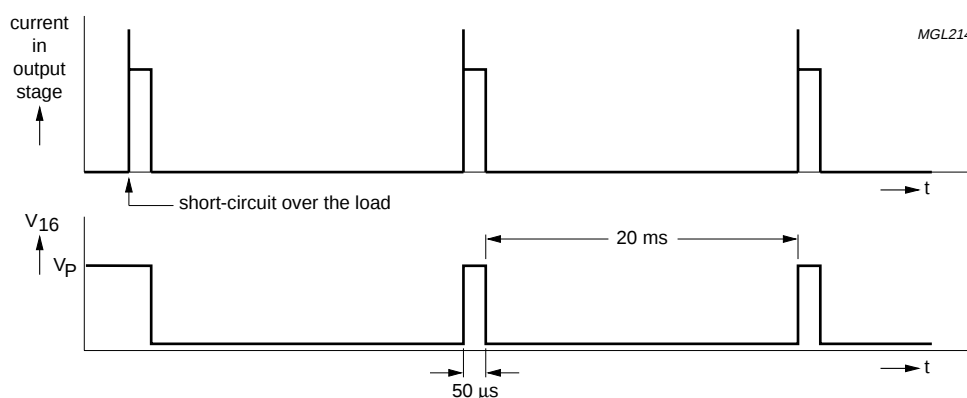
Fig.5 Short-circuit waveform.
