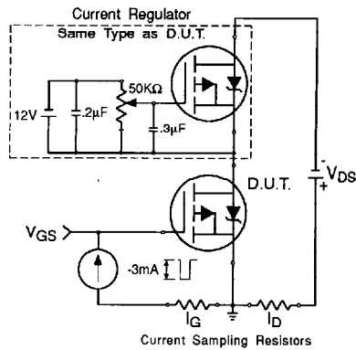
Fig 22b. Gate Charge Test Circuit
