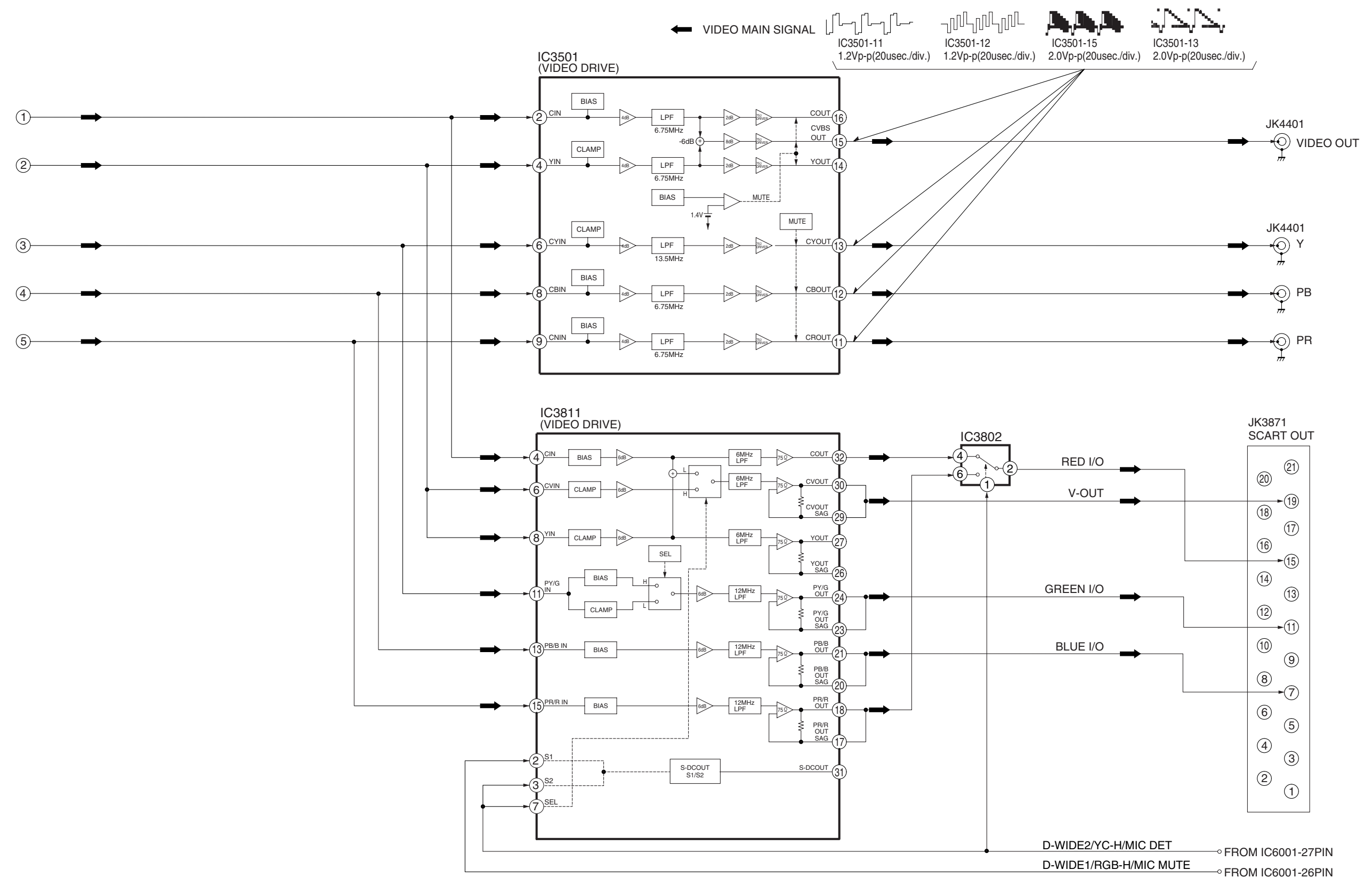
DVD-S42EE VIDEO BLOCK DIAGRAM
