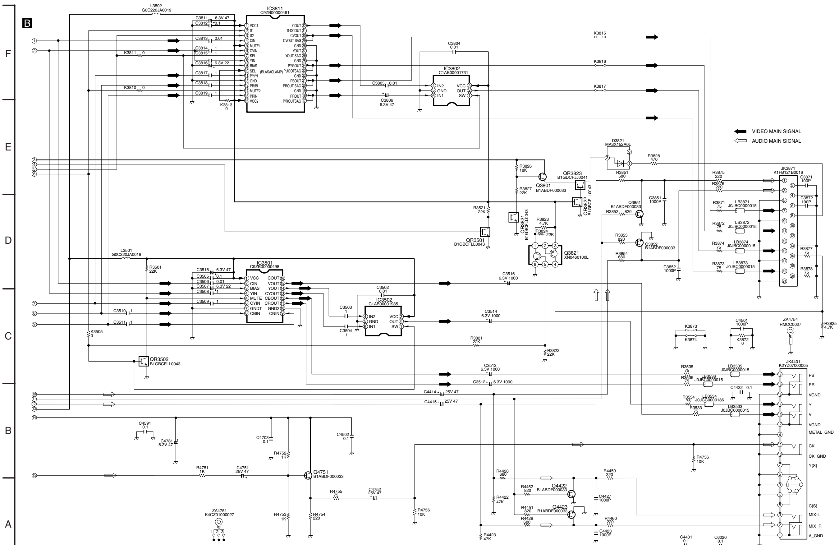
DVD-S42EE FRONT & AV OUT SECTION (MOTHER P.C.B.(2/2)) SCHEMATIC DIAGRAM
