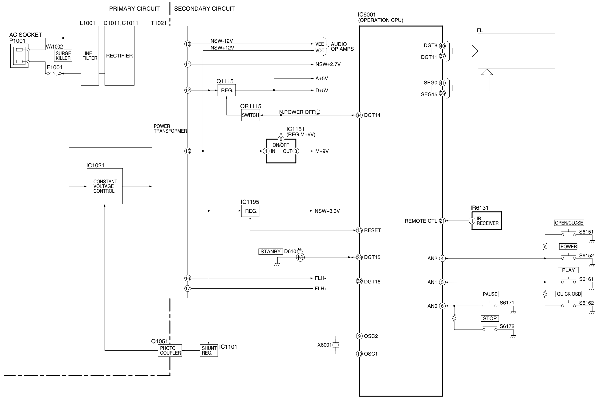
DVD-S42EE/GC/GCA/GCS/GCU/PL/PLA POWER SUPPLY BLOCK DIAGRAM
