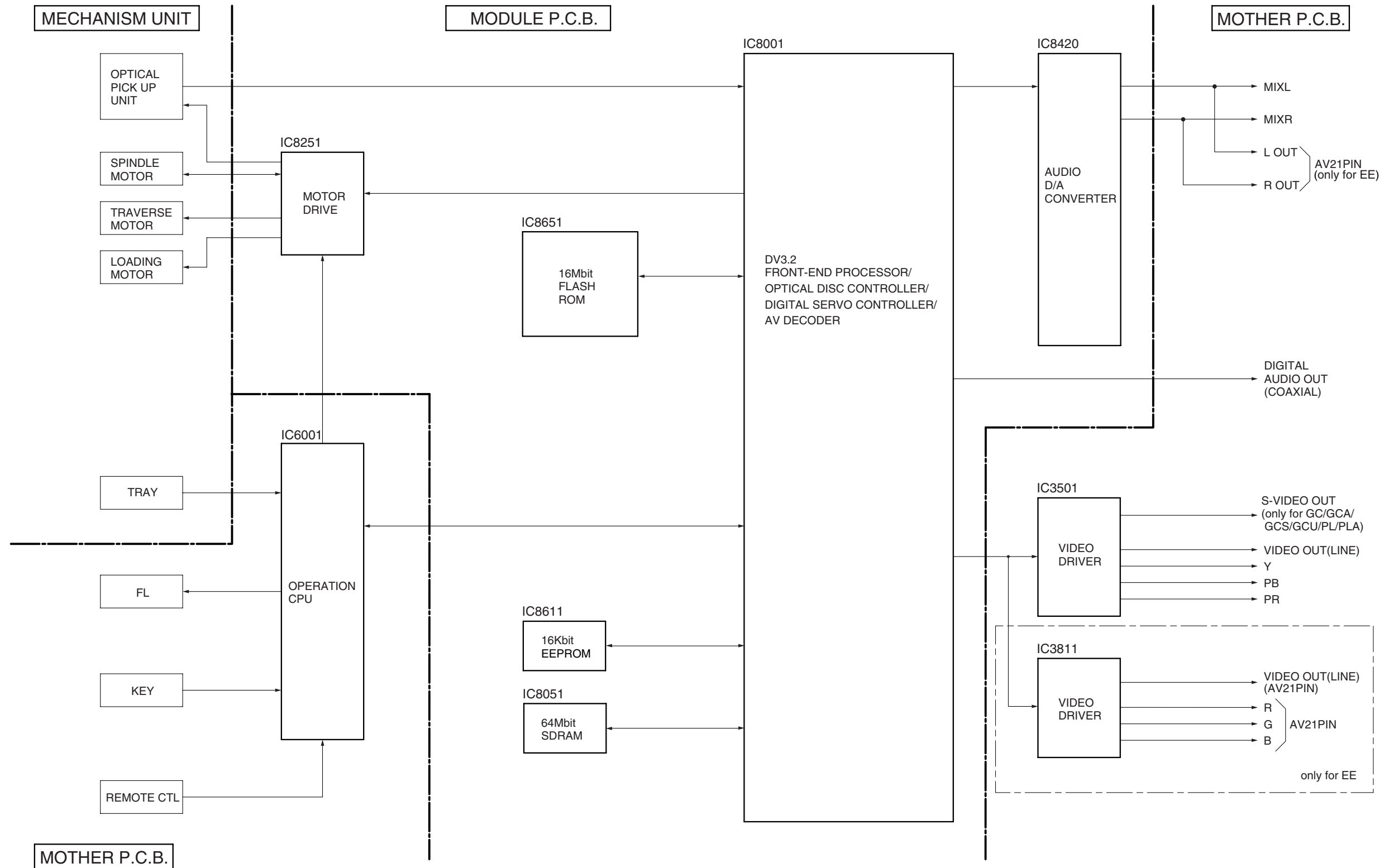
DVD-S42EE/GC/GCA/GCS/GCU/PL/PLA OVERALL BLOCK DIAGRAM
