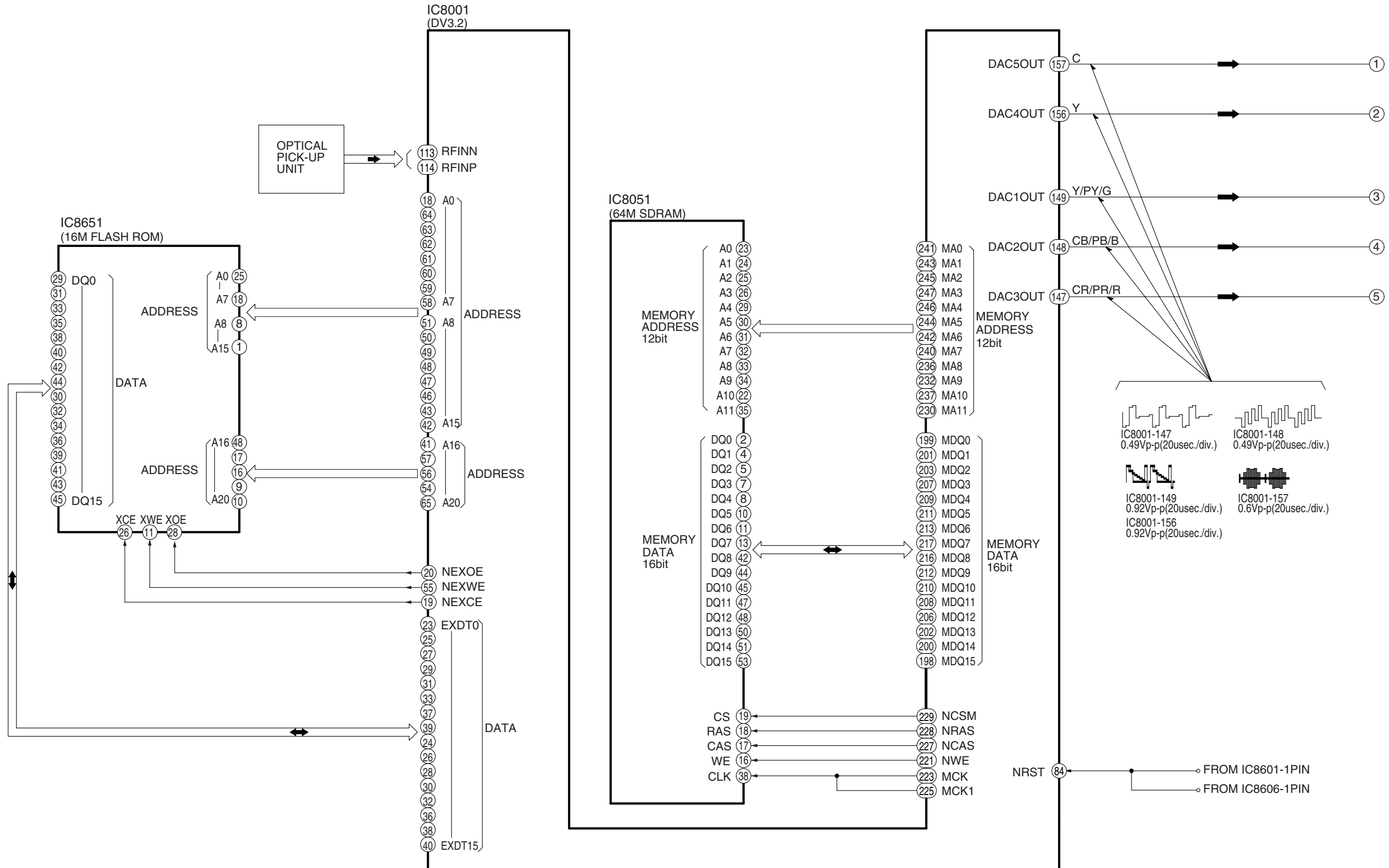
DVD-S42EE VIDEO BLOCK DIAGRAM
