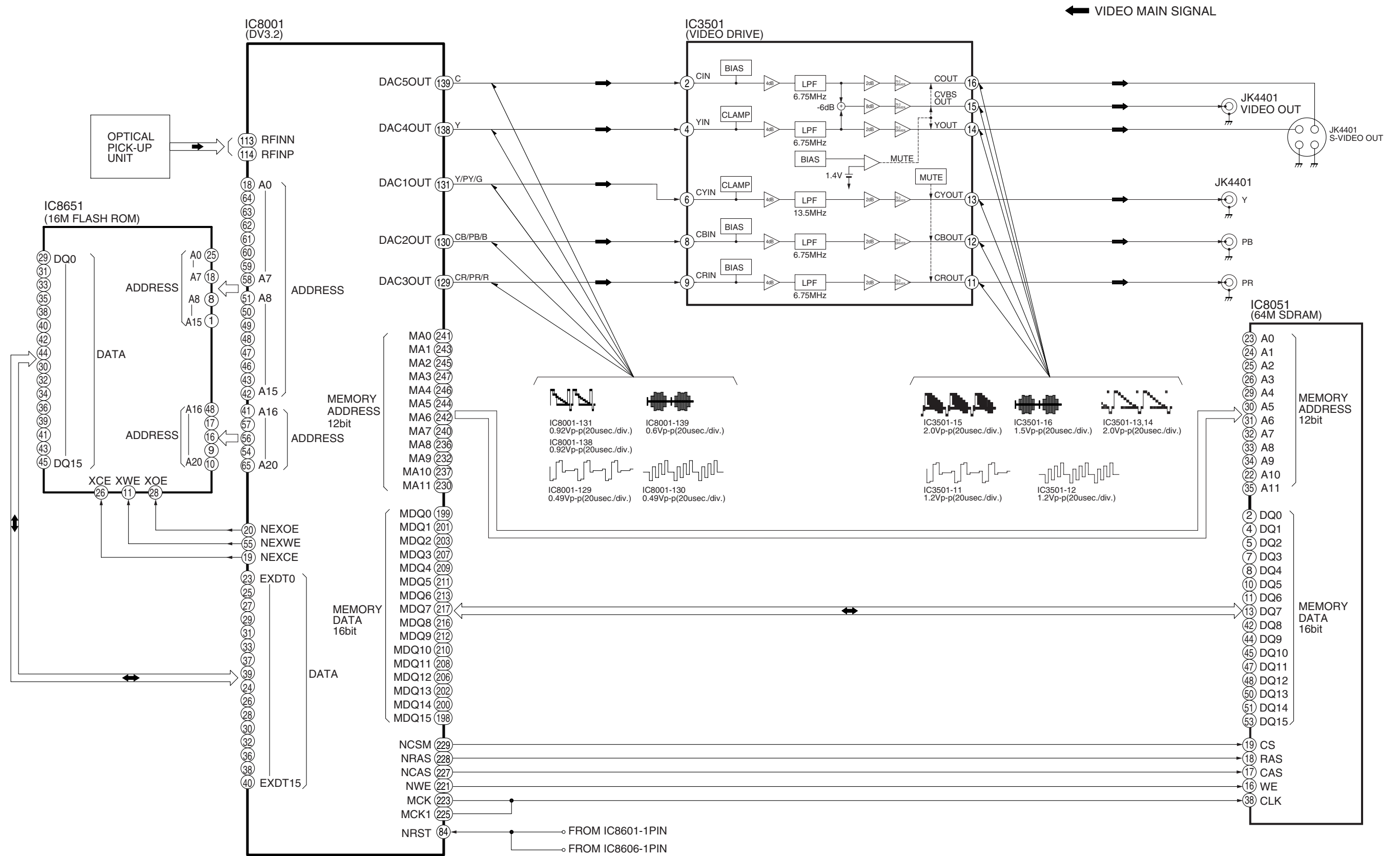
DVD-S42GC/GCA/GCS/GCU/PL/PLA VIDEO BLOCK DIAGRAM
