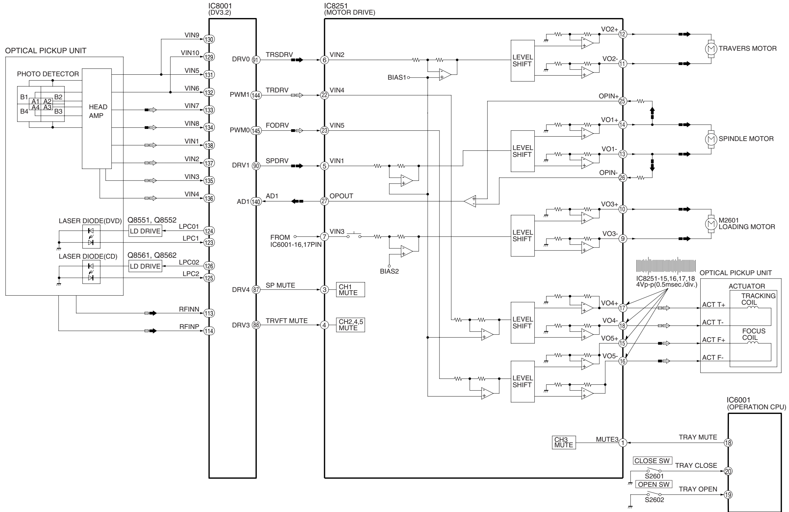
DVD-S42EE/GC/GCA/GCS/GCU/PL/PLA SERVO BLOCK DIAGRAM
