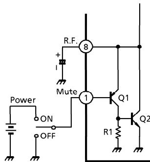
Fig.4 Mute circuit
