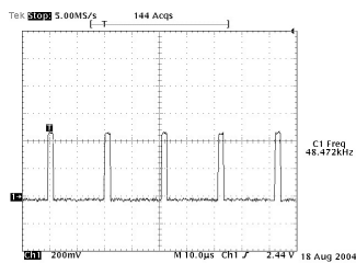
3 R442 H-Sync
