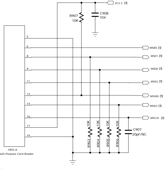
J903-A Multi-Purpose Card-Reader
